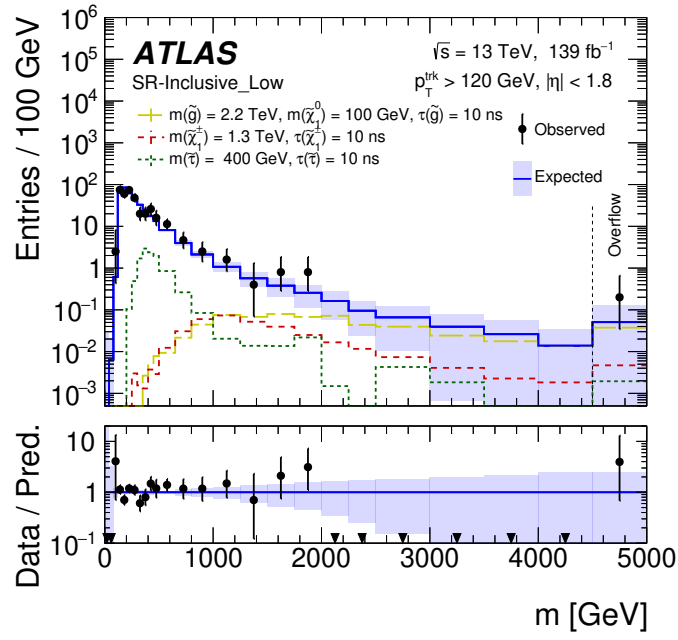
(a) SR-Inclusive_Low
