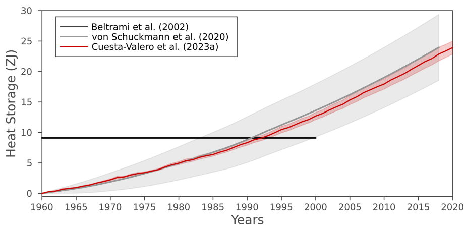
Figure 6. Continental heat storage from Beltrami et al. (2002) (black), von Schuckmann et al. (2020) (gray), and Cuesta-Valero et al. (2023a) (red). Gray and red shadows show the uncertainty range of the heat storage from von Schuckmann et al. (2020) and Cuesta-Valero et al. (2023a), respectively.
