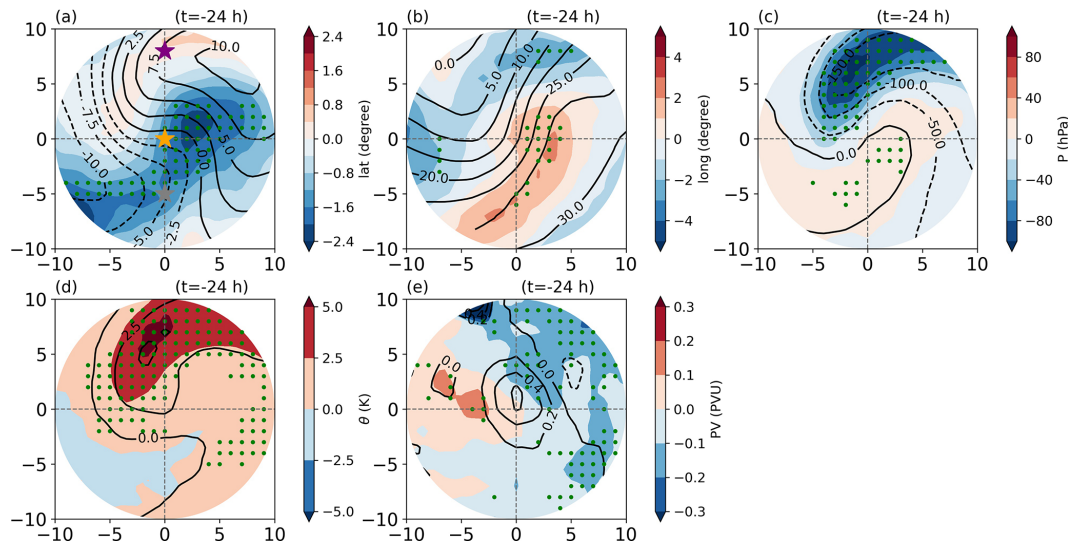
Figure 5. Composites of Lagrangian tendencies along backward trajectories initialized at 250 hPa in the last 24 h before arrival in the cyclone area of (a) latitude, (b) longitude, (c) pressure, (d) potential temperature, and (e) PV. Contours show present-day Lagrangian tendencies, and the color shading indicates the response to future climate change (difference in the Lagrangian tendencies between future and present-day climate). Longitude and latitude are relative to the movement of the cyclone (i.e., with the 24 h longitude and latitude changes of the cyclone center subtracted). Green dots denote regions of ensemble agreement on the sign of change; i.e., more than 80 % of the ensemble members indicate a future change of the same sign. A total of 358 and 308 storms are considered in the present-day and future climate, respectively.
