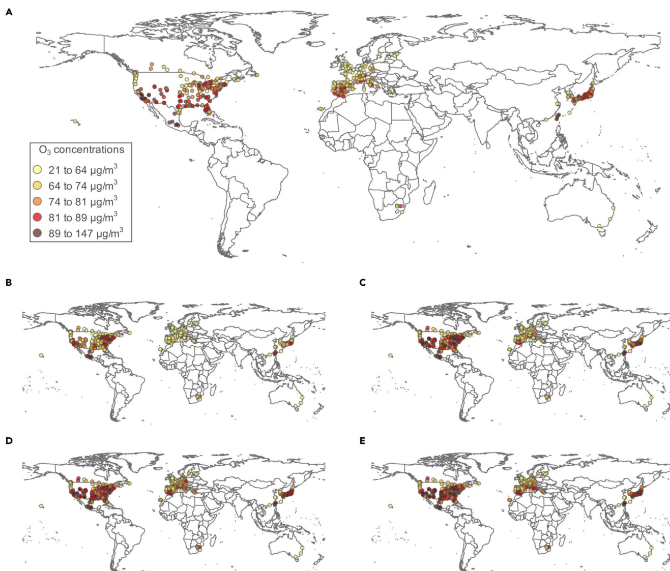
Figure 1. Annual average MDA8 O 3 concentration at 406 locations in 20 countries or regions in present (2010–2014) and future (2050–2054) time periods in the AerChemMIP models (A) Present O 3 concentrations in each city, (B) absolute change in O 3 concentrations under SSP1-2.6, (C) absolute change in O 3 concentrations under SSP2-4.5, (D) absolute change in O 3 concentrations under SSP3-7.0, and (E) absolute change in O 3 concentrations under SSP5-8.5. O 3 concentration is the maximum daily 8-h average.
