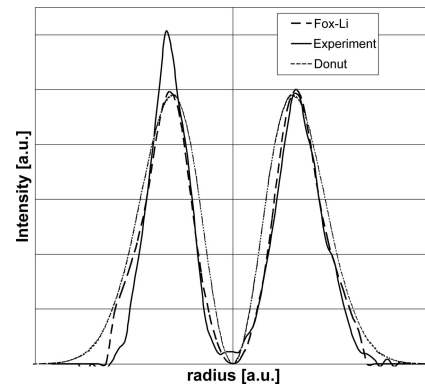
Fig. 8. Horizontal cross section of the radially polarized doughnut mode. Comparison of the experimental data, the theoretical TEM 01 mode, and the Fox–Li simulation taking the diffraction losses into account.
