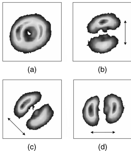
Fig. 7. Intensity distribution of the radially polarized CO 2 laser beam: (a) without polarizer, and through a polarizer oriented (b) vertically, (c) at 45°, and (d) horizontally.
