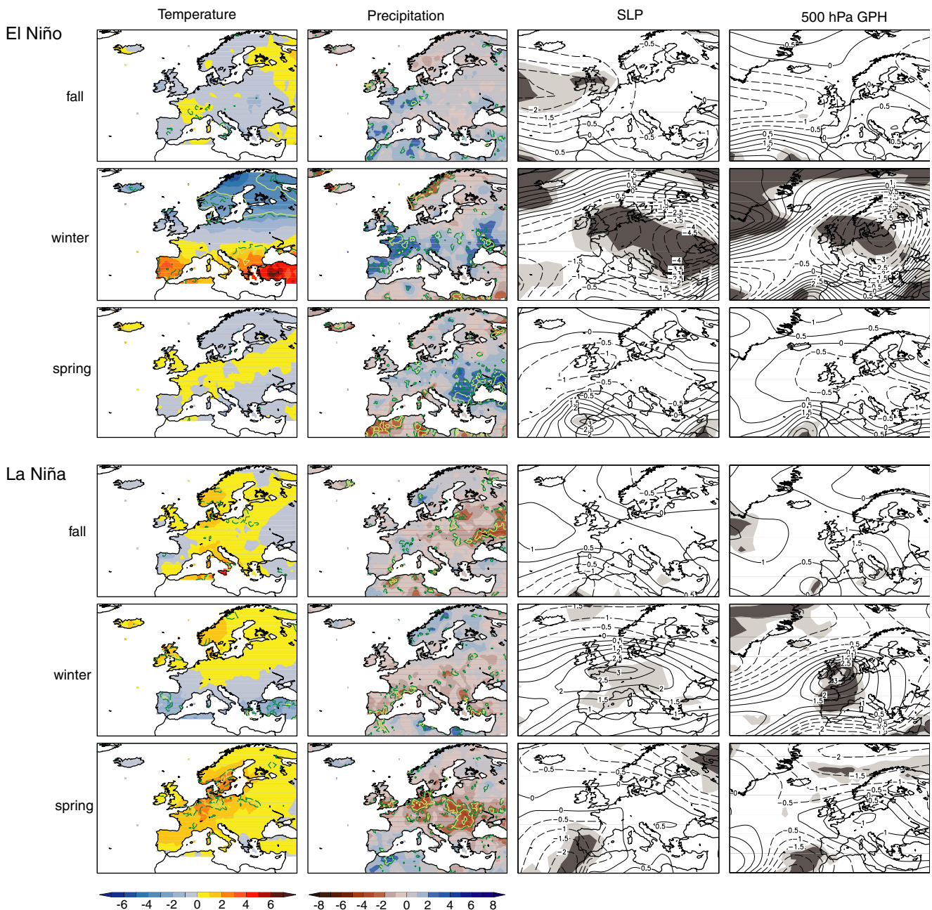
Fig. 3 Composite anomaly fields (scaled means, modified t -values; see text for details) of temperature, precipitation, sea-level pressure ( SLP ) and 500 hPa geopotential height ( GPH ) for different seasons during strong El Niño and La Niña events in the period INS (1880–2003, volcanically perturbed winters were excluded). Note that fall, winter and spring refer to OND, JFM
