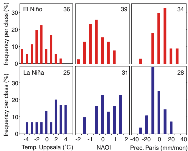
Fig. 6 Histograms of January-to-March averages of temperature at Uppsala ( left , since 1722), the North Atlantic Oscillation (NAO) index ( middle , 1706) and precipitation in Paris ( right , 1706) for strong El Niño events ( top , red ) and strong La Niña events ( bottom , blue ). Volcanically perturbed winters were excluded. The number of cases is given in the top right corner
