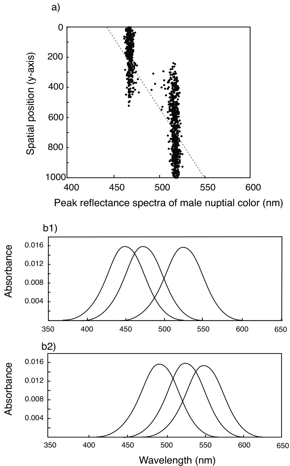
Figure 1 Spatial distribution of individuals and the reflectance spectra of male nuptial colors after speciation occurred (a) and the absorption spectra of three visual pigments (SWS, MWS and LWS) for two individuals which are reproductively isolated (b1 and b2). Broken line indicates environmental wavelength to which individuals can adapt.
