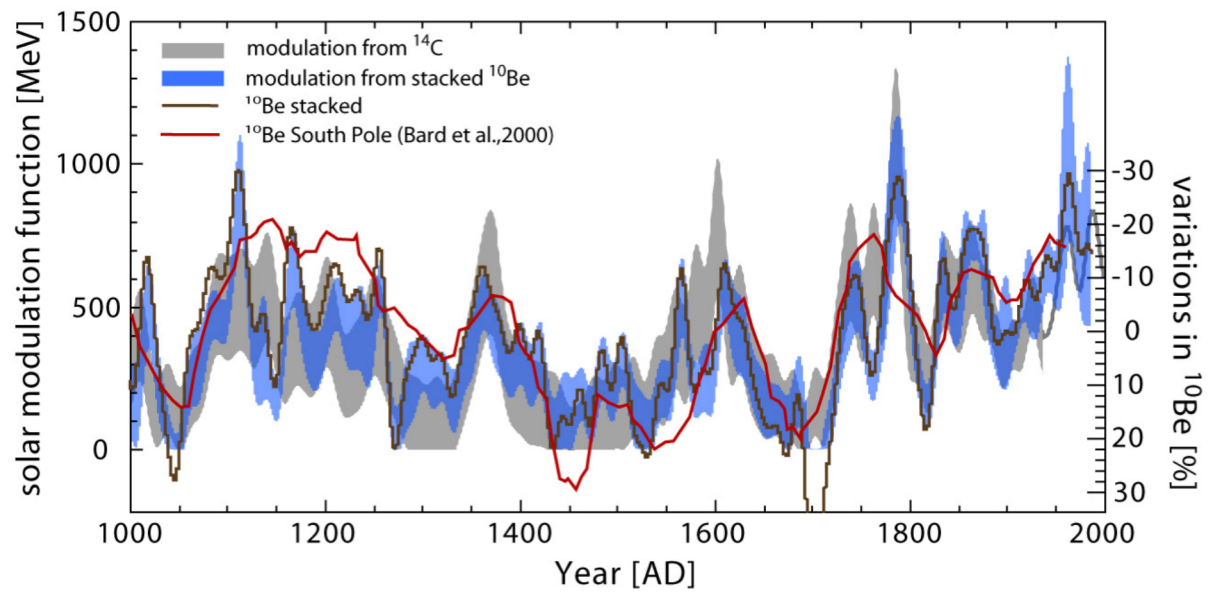
Figure 1: Summary of our results and differences to the South Pole record that underlies Bard et al.'s analysis. The grey band shows the most likely ^{14}\text{C} -based solar modulation record (Figure 6b in Muscheler et al., 2007). The blue band shows the solar modulation from the stacked ^{10}\text{Be} record (without “outlier” and corrected for a slight polar bias according to Field et al., 2006). The uncertainty bands indicate \pm 1 standard deviations arising from uncertainties in the radioisotope records and in the geomagnetic field. Reconstructed modulations are higher, but still within the uncertainty band, when applying the model-based geomagnetic reconstruction of Korte and Constable (2005) instead the Yang et al. data. Usually, the reconstructions agree within uncertainties although not all ^{10}\text{Be} peaks can be trusted as real changes in solar activity. However, the composite ^{10}\text{Be} and ^{14}\text{C} solar modulation records confirm variations (e.g. around 1800 AD) that are not present in the South Pole record. Variations in the ^{10}\text{Be} concentration in ice (right scale) are shown for the stacked and low-pass filtered ^{10}\text{Be} record where “outliers” were removed (brown) and the smoothed South Pole ^{10}\text{Be} record from Bard et al., 2000 (red).
