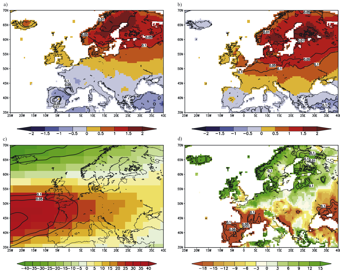
Figure 2. Anomaly composite of the European winter temperature [ ^{\circ}\text{C} ] in (a) year 0 and (b) year 1 following 15 tropical volcanic eruptions over the past half millennium. Anomaly composite of (c) the European winter 500 hPa geopotential height anomaly [gpm] and (d) winter precipitation [mm/month] in year 1 following 10 tropical volcanic eruptions over the past half millennium. The black contours mark the statistical significance as p-values (representing 90%, 95% and 99% confidence level) of the Mann-Whitney Rank Sum Test.
