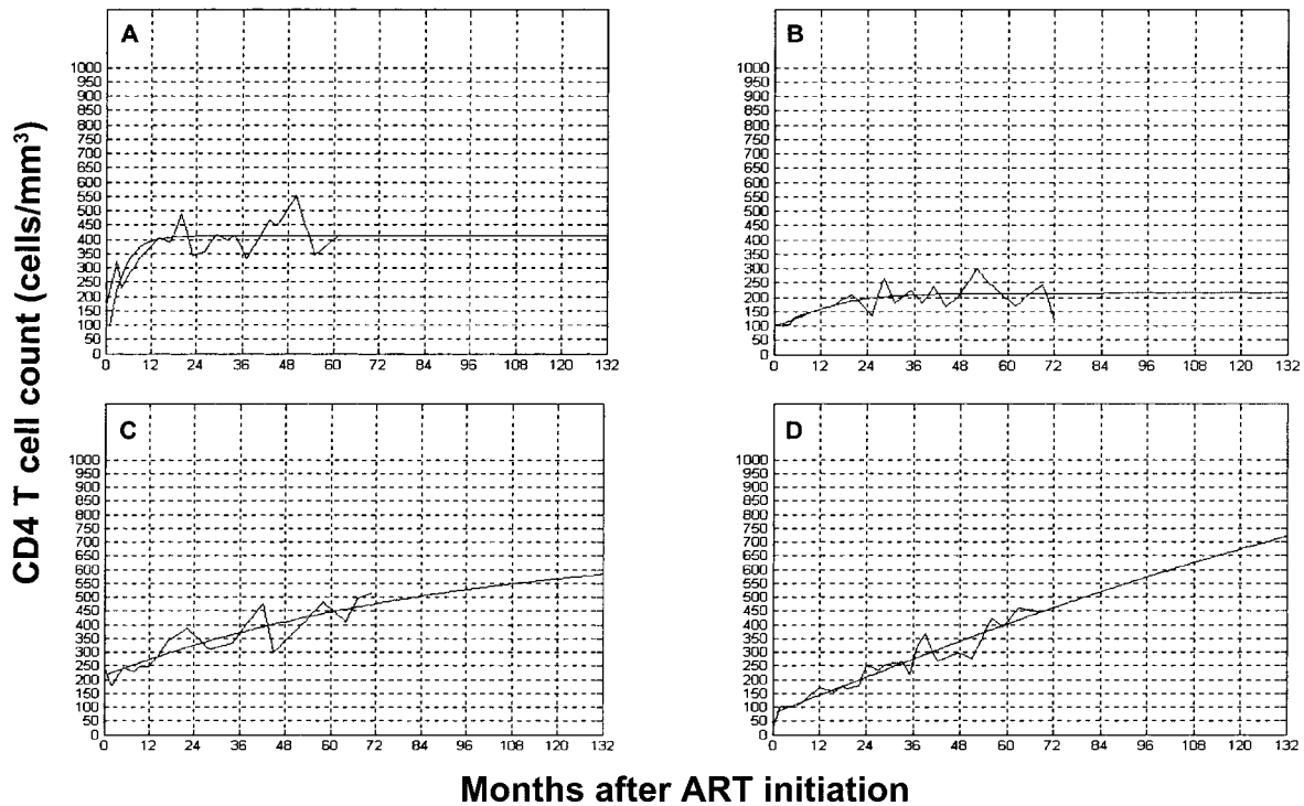
Figure 3. Distinct patterns of CD4 T cell recovery in 4 patients for whom the CD4 T cell count reached a plateau <500 cells/ \mu L (A and B) or showed a slow, but steady increase (C and D).
