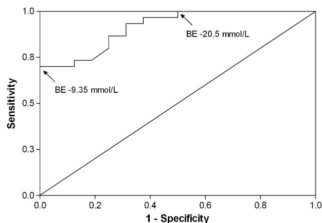
Figure 3. Receiver operating characteristic (ROC) curve for base excess (BE) 1 h after admission. The diagonal line corresponds to a test that is sensitive or specific just by chance. The area under the curve is 0.915.
