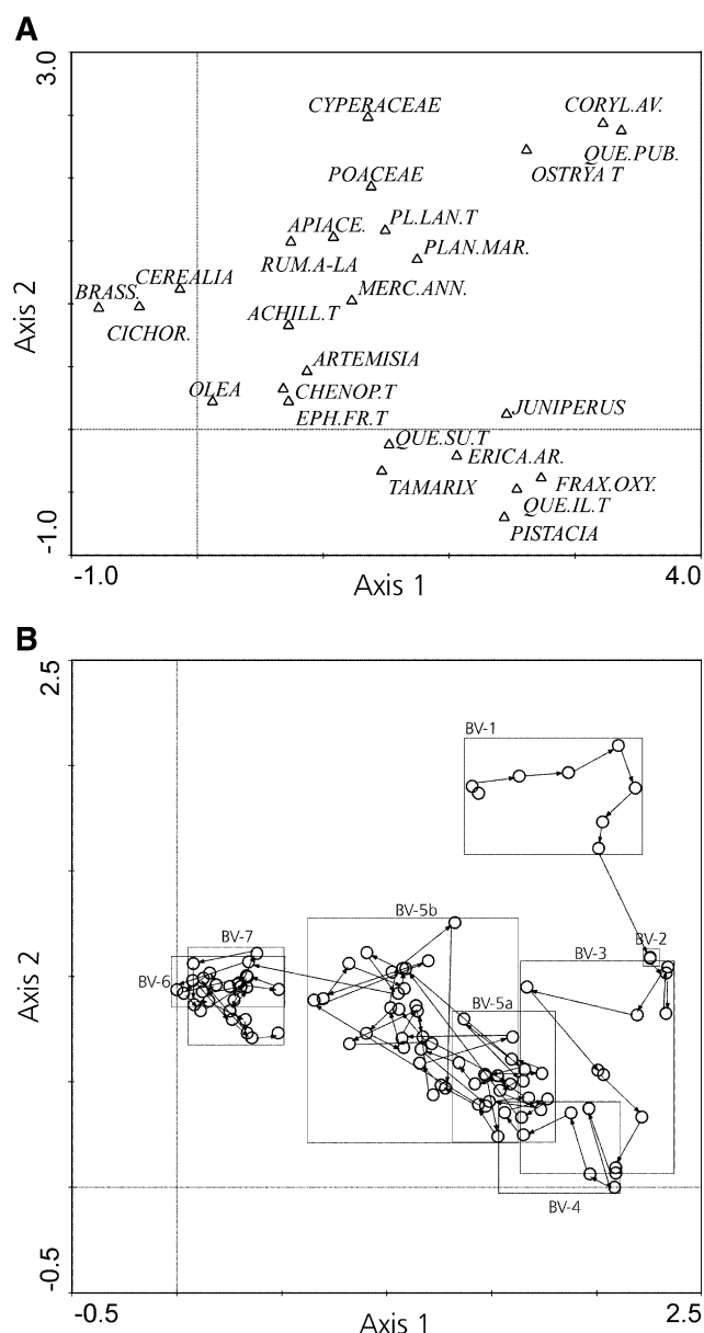
Fig. 7 Sample and species scores of DCA analysis. a DCA- axes 1 and 2 of species scores. b DCA- axes 1 and 2 of sample scores. Rectangles show LPAZ of Biviere di Gela according to optimal partitioning and b-stick analyses
