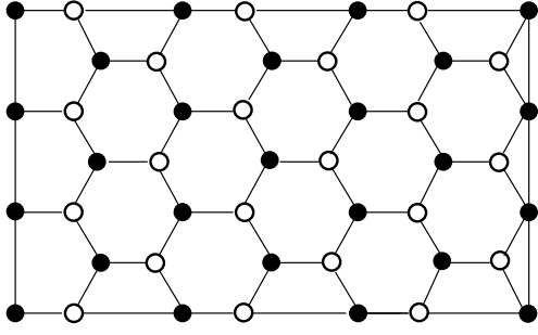
Fig. 1. Bipartite non-Bravais honeycomb lattice consisting of two triangular Bravais sublattices.
