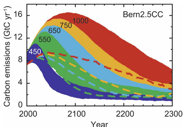
FIG. 10. Projected allowable carbon emissions leading to stabilization of atmospheric \text{CO}_2 at different levels and the effects of uncertainty in carbon cycle processes on calculated emissions as projected with the Bern2.5CC EMIC. Uncertainties in the carbon cycle processes for the Bern2.5CC EMIC are calculated as in IPCC TAR (see the text and appendix A for details). Dashed lines highlight the lower bounds of the uncertainty ranges for individual profiles if otherwise hidden. Results are 31-yr running averages.
