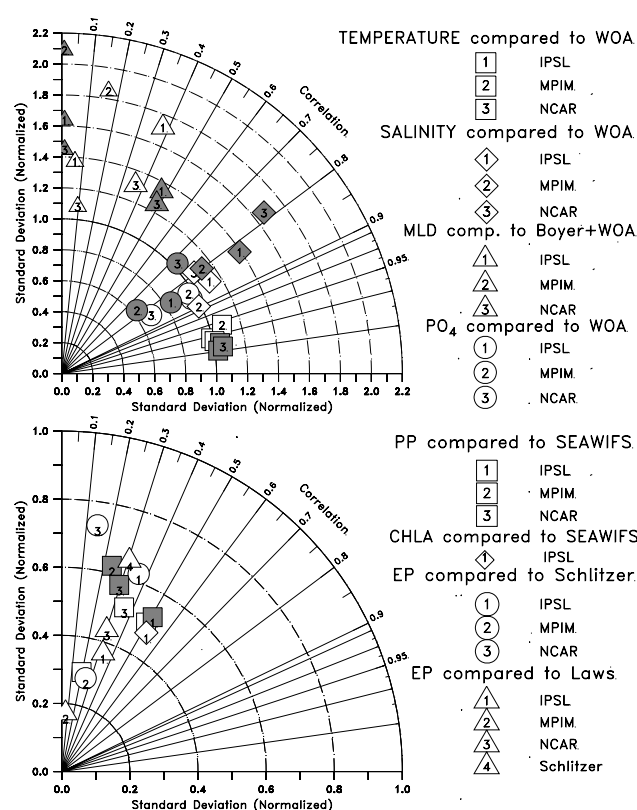
Fig. 1. Top: Taylor diagram showing the correspondence between model results and observations for 3-D fields weighted by volume of annual mean temperature (squares), salinity (diamonds) and PO 4 3- concentration (circles), as well as 2-D fields of MLD (small and large triangles). White symbols indicate annual mean values, except for MLD where they represent the respective maximum (MLD max ). Grey symbols show spatial correlations including the seasonal cycle of sea surface temperature (SST), sea surface salinity (SSS), PO 4 3- (averaged over 0–100 m) and MLD. Modelled MLD is compared to data from de Boyer-Montégut et al., (2004) (large triangles) and based on a recalculation (small triangles) from T and S from the models and data from the World Ocean Atlas (WOA; Collier and Durack, 2006; Conkright et al., 2002). For MPIM the normalised standard deviation of MLD compared to de Boyer-Montégut et al., (2004) is 6.0 and 4.7 for MLD max and seasonal MLD, respectively, and therefore not displayed in the diagram. Bottom: Taylor diagram showing the correspondence between model results and observation-based estimates for primary production (PP; squares), chlorophyll (CHLA; diamond) and particulate organic carbon (POC) export production (EP; circles and triangles). White symbols show results for annual mean 2-D fields, grey symbols include the seasonal cycle for PP. The angular coordinate indicates the correlation coefficient ( R ), the radial coordinate shows the normalised standard deviation ( \text{std}_{\text{model}}/\text{std}_{\text{obs}} ). A model perfectly matching the observations would reside in point (1,1).
