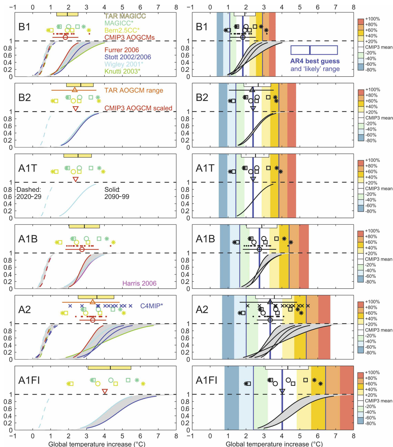
FIG. 2. Global-mean temperature projections for the six illustrative SRES scenarios. (left) The CDFs for global-mean surface air temperature increase for short-term (2020–29, dashed) and long-term (2090–99, solid) projections relative to the 1980–99 average are shown at bottom of each plot. Different colors mark different models or statistical methods. Lines are only shown from the 5% to the 95% level, thus the horizontal dimension of each curve marks the 5%–95% confidence range. Light gray shading marks the envelope of all CDFs. Labels with asterisks indicate that the respective method considers carbon cycle–climate feedback uncertainties. Other estimates of uncertainty for 2090–99 are shown at the top of each plot. Central values and ranges are given as means and 5%–95% from a fitted normal distribution to the AR4 AOGCM simulations (red circles and lines) for B1, A1B, and A2, along with results for each individual AR4 AOGCM (red dots). For B2, A1T, and A1FI, AOGCM means are estimated using scaling factors from the MAGICC model (red triangles, see text). From the MAGICC simple model (dark green symbols) tuned to 19 AR4 AOGCMs, means (circles) and one standard deviations (squares) are given for fixed carbon cycle parameters (indicating the uncertainty caused by the climate
