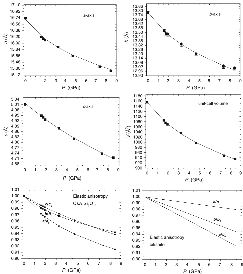
Fig. 4 Variation of the unit-cell parameters of CsAlSi 5 O 12 as a function of pressure with axial and volume III-BM-EoS fit (solid lines) and elastic anisotropy in CsAlSi 5 O 12 and bikitaite (Comodi et al. 2003; Gatta et al. 2003). For a , c and V , the esd values are smaller than the size of the symbols. Notice that in CsAlSi 5 O 12 channels run parallel to the c -axis and in bikitaite parallel to the b -axis
