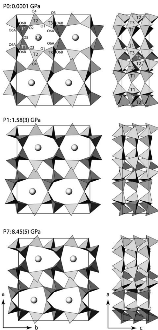
Fig. 3 Unit cell of \text{CsAlSi}_5\text{O}_{12} projected along c -axis (left) and b -axis (right) at P_0 , P_1 and P_7 (top to bottom). Atoms are labelled according to the structural refinements (Table 1). For easier illustration, Cs is not shown in the projections along the b -axis. A drastic structural change occurs between P_0 to P_1 : O5 is shifted along the c -axis due to rigid-body tetrahedral rotation
