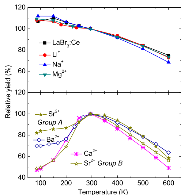
FIG. 6. Temperature dependence of the relative photoelectron yield of standard LaBr 3 :Ce and LaBr 3 :Ce co-doped samples with Li, Na, Mg, Ca, Sr, and Ba. The spectra are normalized to 100% at 295 K.
