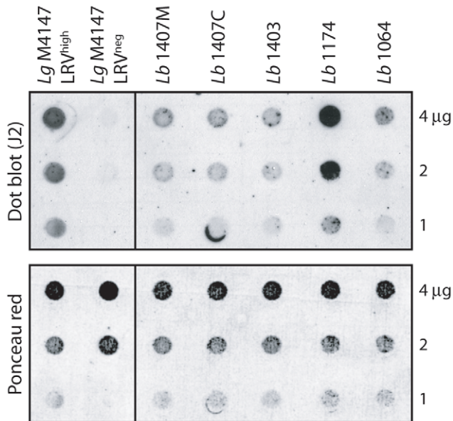
Figure 6. Screening for LRV in human isolates of Leishmania . Parasites of 5 different L. braziliensis strains previously shown to harbor LRV [24] were analyzed by dot blot (1 to 4 \mu g total protein/spot). doi:10.1371/journal.pntd.0002006.g006
