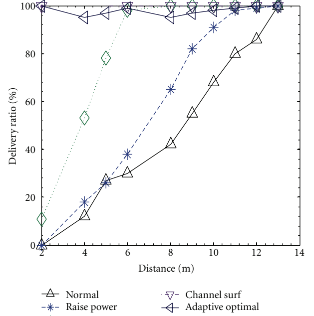
FIGURE 3: Delivery ratio of different strategies.
