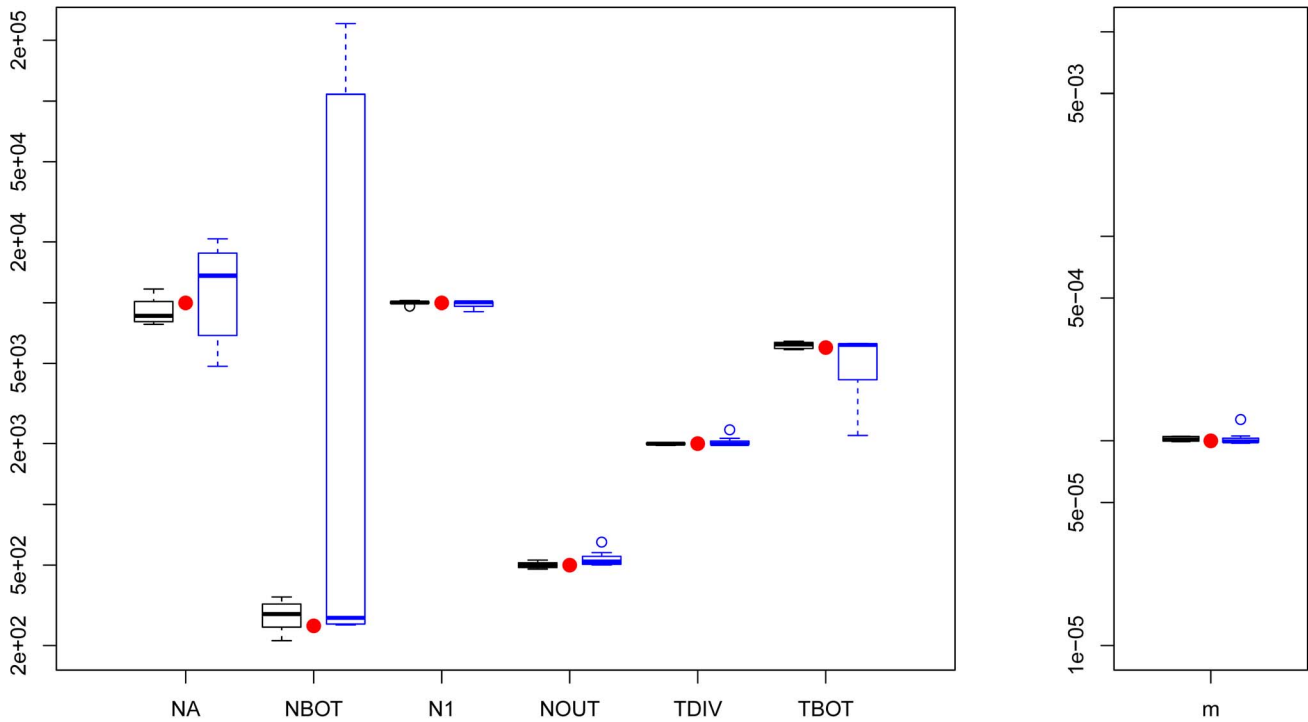
Figure 2. Three population divergence and growth model. fastsimcoal2 results are in black and daði 's results (8/10) are in blue. True parameters values are shown as red dots. fastsimcoal2 required 4–5 h for a single estimation based on 40 ECM cycles over parameters, whereas a run of daði requires on average 34 hours on a similar CPU. doi:10.1371/journal.pgen.1003905.g002
