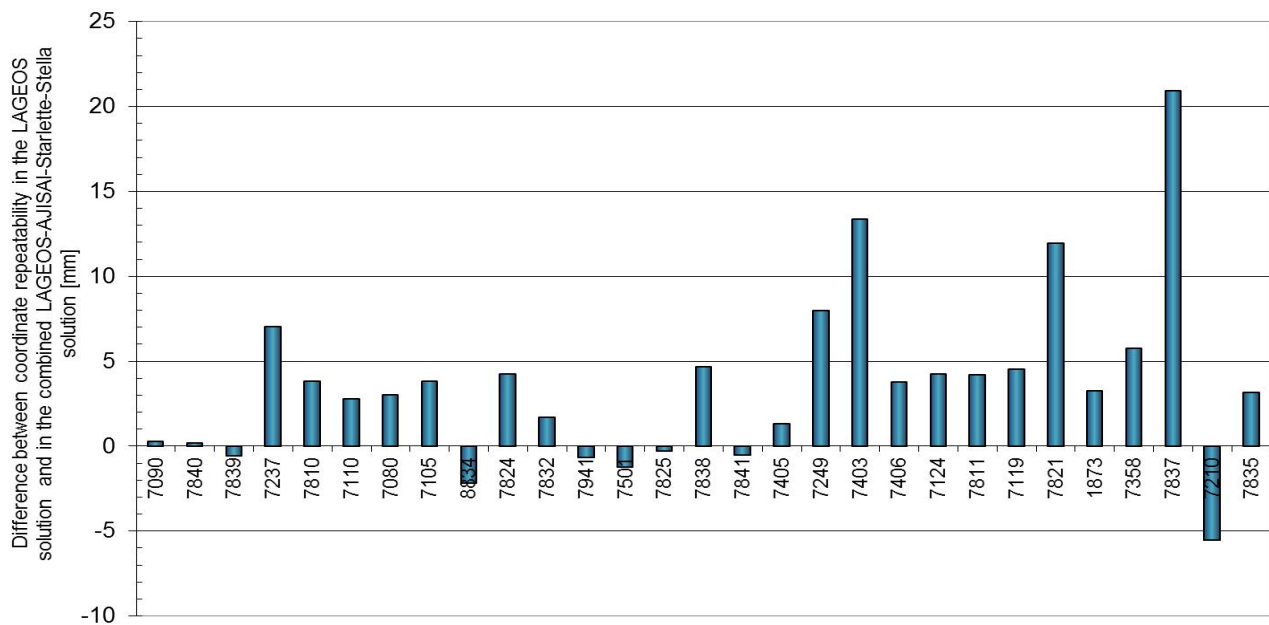
Figure 3. Difference between coordinate repeatability in the LAGEOS-1/2 solutions and in the multi-SLR solutions, after Sošnica et al., (2013b).
