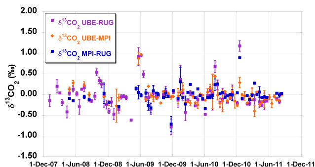
Fig. 7. Differences of the \delta^{13}\text{CO}_2 values measured by each pair of two laboratories. The average differences are: -0.03\text{‰} for UBE-RUG, -0.02\text{‰} for UBE-MPI and -0.02\text{‰} for MPI-RUG. The error bars represent the quadratically added standard errors of the measurements of the two laboratories.
