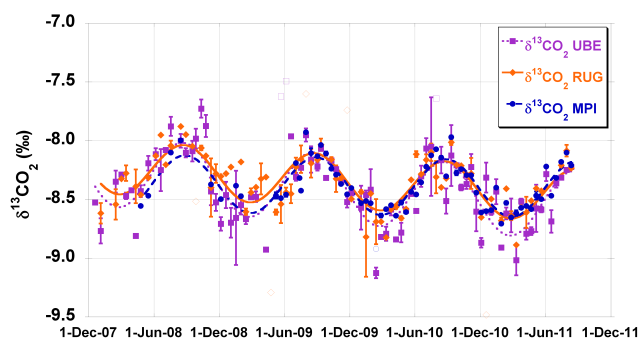
Fig. 6. \delta^{13}\text{CO}_2 observations from Jungfraujoch, Switzerland from flask samples measured by three laboratories: UBE (pink squares), RUG (orange diamonds) and MPI (blue circles). The values are the averages of 1, 2 or 3 flasks. The fits through the data are linear trend plus single harmonic seasonal components. Open symbols represent those values that are outliers to the fit of the individual data set (based on the 2.7 sigma exclusive filter on the residuals). The error bars represent the standard error of the average value of 2 or 3 flasks. For single flask measurements error bars are not shown.
