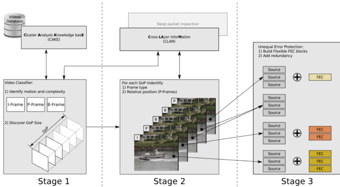
Figure 1.9. ViewFEC stages [Immich et al. 2013]
