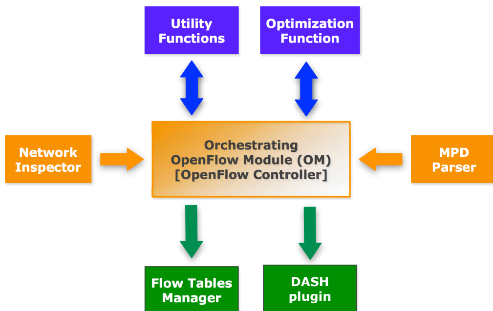
Figure 1.12. OpenFlow-assisted QoE Fairness Framework [Georgopoulos et al. 2013]
