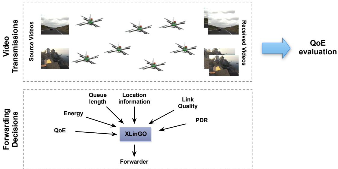
Figure 1.10. XLinGO forwarding decisions
