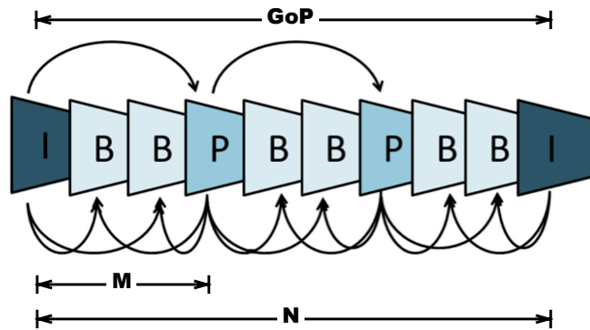
Figure 1.6. Group of Pictures Structure
