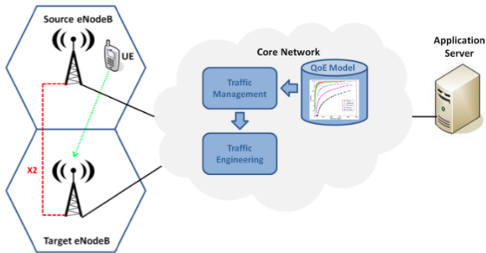
Figure 1.11. QoE-aware multi-cell handover scenario [Shehada et al. 2013]
