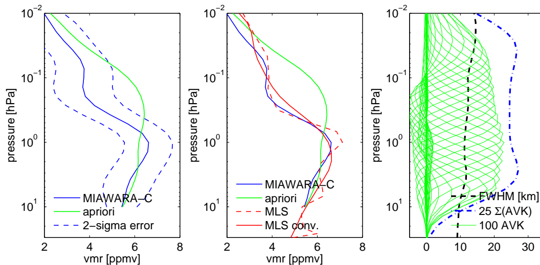
Fig. 12. Water vapor profile retrieved from the one day spectrum shown in Fig. 11 plotted together with the a priori profile and the upper limit for the systematic plus random 2\text{-}\sigma error and compared to the profile of a close MLS overpass ( 67.5^\circ\text{ N} , 21.0^\circ\text{ E} ) in the middle plot. The averaging kernels of MIAWARA-C are shown on the right together with the FWHM and the sum of each of the kernels.
