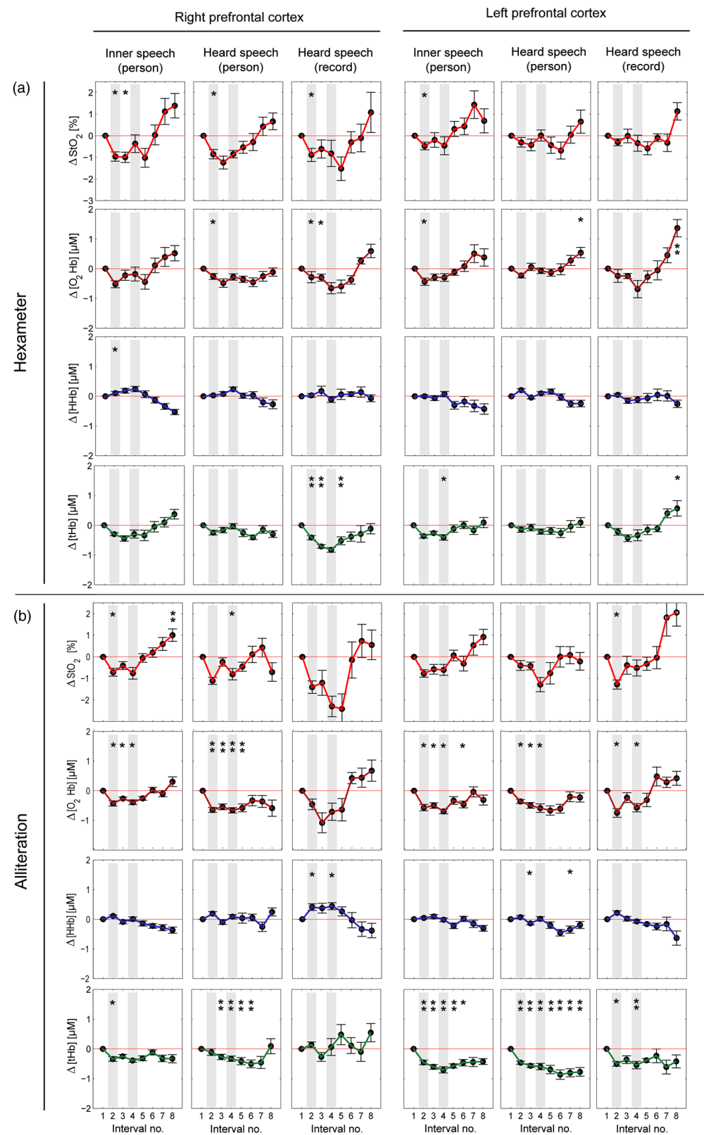
Fig. 2 Changes in StO_2 , [O_2Hb] , [HHb] , and [tHb] over the course of the experiments. Each interval refers to a time span of 3 min. The shaded areas indicate the periods when the tasks were performed. All data are shown as median values (black circles) \pm standard error of the median ( SE_{median} = MAD/n^{0.5} , where MAD is the median absolute deviation and n is the number of measurements). Significant changes are marked with an asterisk: p < 0.05 (*). Corrected significant p -values (according to the Benjamini-Hochberg correction) are marked with two vertically aligned asterisks.
