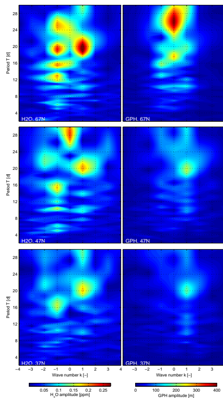
Fig. 4. Periodogram for travelling and stationary planetary waves in water vapor (left panels) and geopotential height (right panels) on 0.05 hPa (approximately 70 km) as observed by Aura MLS at the latitudes of the ground based microwave radiometers (67° N, 47° N and 37° N, from top to bottom) during boreal winter 2011/2012.
