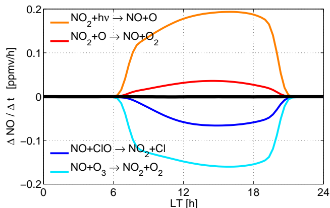
Figure 3. Zonal-mean conversion rates of NO at 5 hPa, 21 March, 50° N. The corresponding reactions are given next to the conversion lines. The net conversion rate of NO (black line) shows negligible conversion rate since common NO changes at the solar terminator are from 0 to approximately 10 ppbv. Reactions with absolute conversion rates less than 5 ppbv h -1 are omitted.
