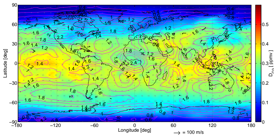
Figure 7a. Monthly mean modelled DO_3 at 5 hPa in March as a function of longitude and latitude. A daytime average of horizontal wind (grey arrows) from 09:00 to 15:00 LT is overlaid and a reference for wind speed is given near the x axis. The magenta contour lines refer to the peak-to-valley difference D_T in temperature given in K.
