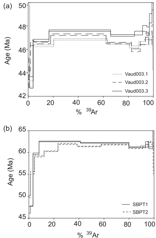
Fig. 8. (a) Age spectra of samples Vaud003.1, Vaud003.2 and Vaud003.3; the sieved size fractions are 125–160 \mu\text{m} , 160–250 \mu\text{m} and 250–500 \mu\text{m} , respectively. The age spectra are almost parallel, with an age difference of \approx 0.5 Ma. (b) Age spectra of samples SBPT1 and SBPT2; the size fractions are 160–500 \mu\text{m} and 125–160 \mu\text{m} respectively. The two age spectra coincide within 1 Ma over 80% of the ^{39}\text{Ar} release.
