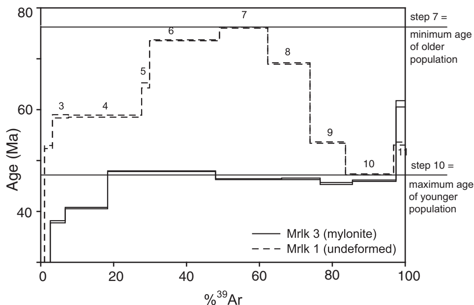
Fig. 9. ^{39}\text{Ar} – ^{40}\text{Ar} age spectra of two samples from the Bottarello glacier, Monte Rosa nappe. Both samples belong to the same host-rock and were collected 1 m apart. Mrlk1 shows an upward-convex age spectrum, typical of a mixture of two diachronous white micas. Mrlk3 shows a much flatter age spectrum between 48 and 46 Ma. The coincidence of the plateau age of Mrlk3 with the maximum age for the younger population of Mrlk1 suggests that the same c. 48 Ma mica population that predominates in Mrlk3 is also present in Mrlk1, but not exclusively. The behaviour of the ^{39}\text{Ar} – ^{40}\text{Ar} isotopic system cannot be explained by thermal criteria and can be correctly predicted only by the microstructural observation that mylonite sample Mrlk3 almost exclusively consists of Alpine mica, whereas Mrlk1 was little deformed during the Alpine orogeny. Keller et al. (2004) observed pre-Alpine relicts only in Mrlk1.
