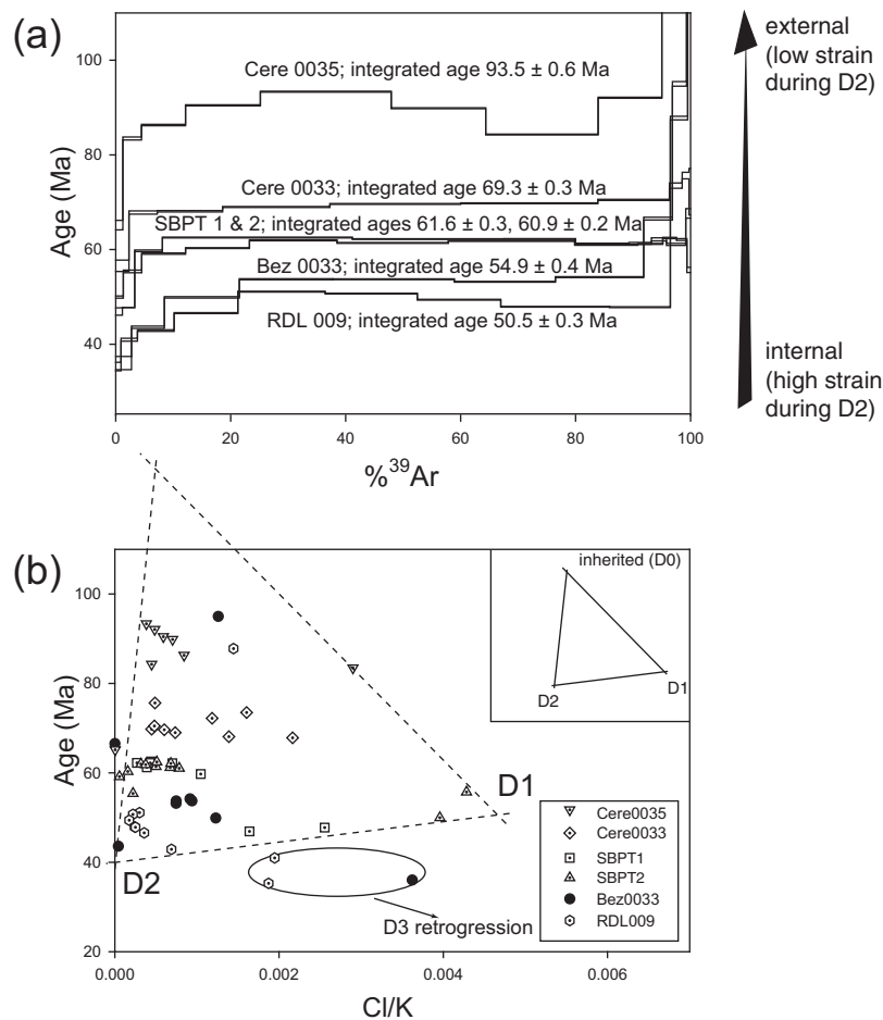
Fig. 11. ^{39}\text{Ar} - ^{40}\text{Ar} results from the Rutor Unit. (a) Age spectra of all samples from the Rutor Unit. The relationship between structural position and integrated age should be noted. The apparent 'plateaux' of samples SBPT1 and Bez0033 are geologically meaningless, as they represent mixtures between Alpine metamorphic mica and an inherited component. (b) Cl/K-age correlation diagram. The three vertices point to an age of 47 \pm 1 Ma for D_1 , 40 \pm 1 Ma for D_2 and an inherited component with a geologically meaningless apparent age of about 135 Ma. The three youngest step ages are interpreted as Cl-rich D_3 retrogression.
