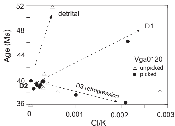
Fig. 12. ^{39}\text{Ar} - ^{40}\text{Ar} results from the Internal Unit: Cl/K-age correlation diagram for syn- D_2 mylonite sample Vga0120 (see age spectrum in Fig. 7b), pointing to a vertex at c. 40 Ma for syn- D_2 mylonitization.
