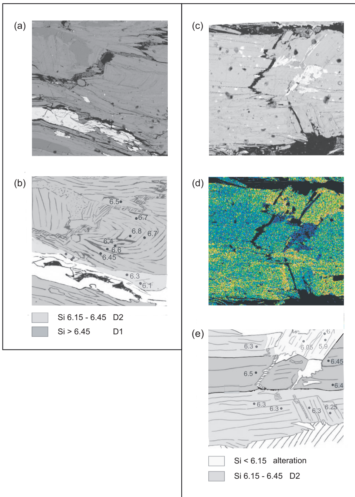
Fig. 6. (a) BSE image of the area shown in Fig. 5b. Field of view 0.3 \times 0.3 mm. (b) Contour map of the Si concentration with individual quantitative analyses. (c) BSE image of the area shown in Fig. 5c. Field of view 0.2 \times 0.2 mm. (d) Al false-colour concentration map; colour coding as in Fig. 4h. (e) Contour map of the Si concentration. It should be noted that although D 1 mica grains and D 2 mica grains show similar orientation they are texturally different, as is visible in Fig. 5.
