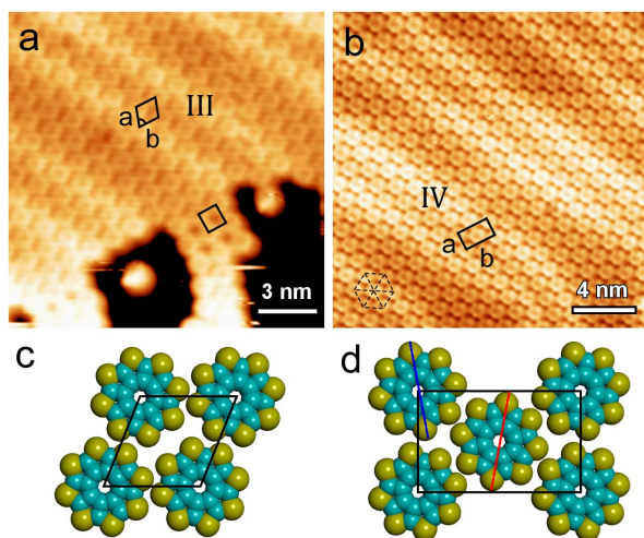
Figure 3 | Intermediate and high coverage phases of 1 on Au(111).
