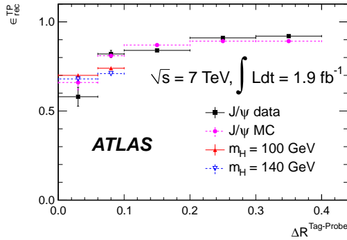
Figure 6: Tag-and-probe reconstruction efficiency \varepsilon_{\text{rec}}^{\text{TP}} as a function of the \Delta R between the two muons, evaluated on a sample of J/\psi \rightarrow \mu^+\mu^- from collision data and a corresponding sample of Monte Carlo events. The \varepsilon_{\text{rec}}^{\text{TP}} for the signal Monte Carlo, evaluated with a similar tag-and-probe method, is also shown. The uncertainties are statistical only.
