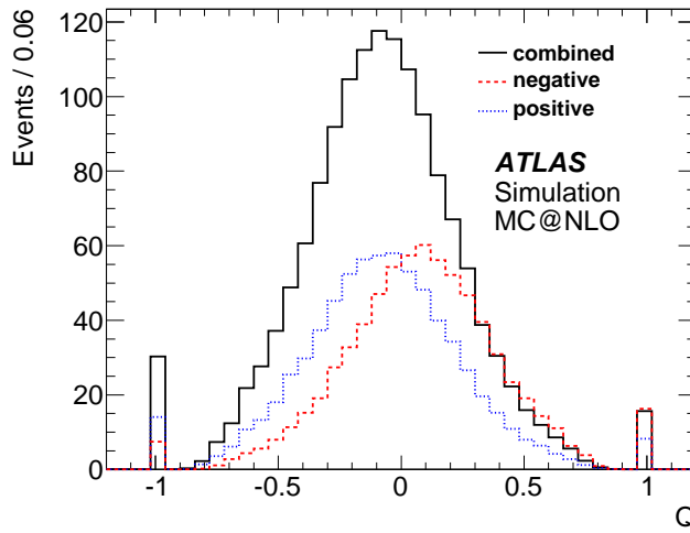
Figure 2. Distributions of the reconstructed b -jet charge in electron+jets t\bar{t} events (MC@NLO) associated with positive (dotted blue line) and negative (dashed red line) leptons and the combined charge (solid black line) after the \ell b -pairing is applied. Here Q represents Q_{b\text{-jet}}^\ell in the first two distributions and Q_{\text{comb}} in the third one.
