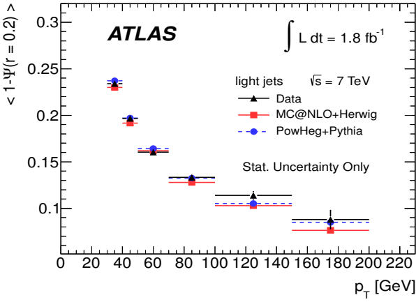
Fig. 8 Dependence of the b -jet (top) and light-jet (bottom) shapes on the jet transverse momentum. This dependence is quantified by plotting the mean value \langle 1 - \Psi(r=0.2) \rangle (the fraction of energy in the outer half of the jet cone) as a function of p_T for jets in the single-lepton sample.
