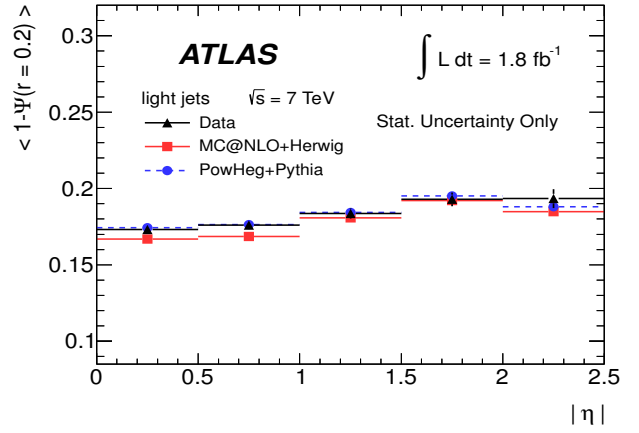
Fig. 9 Dependence of the b -jet (top) and light-jet (bottom) shape on the jet pseudorapidity. This dependence is quantified by plotting the mean value \langle 1 - \Psi(r=0.2) \rangle (the fraction of energy in the outer half of the jet cone) as a function of |\eta| for jets in the single-lepton sample.
