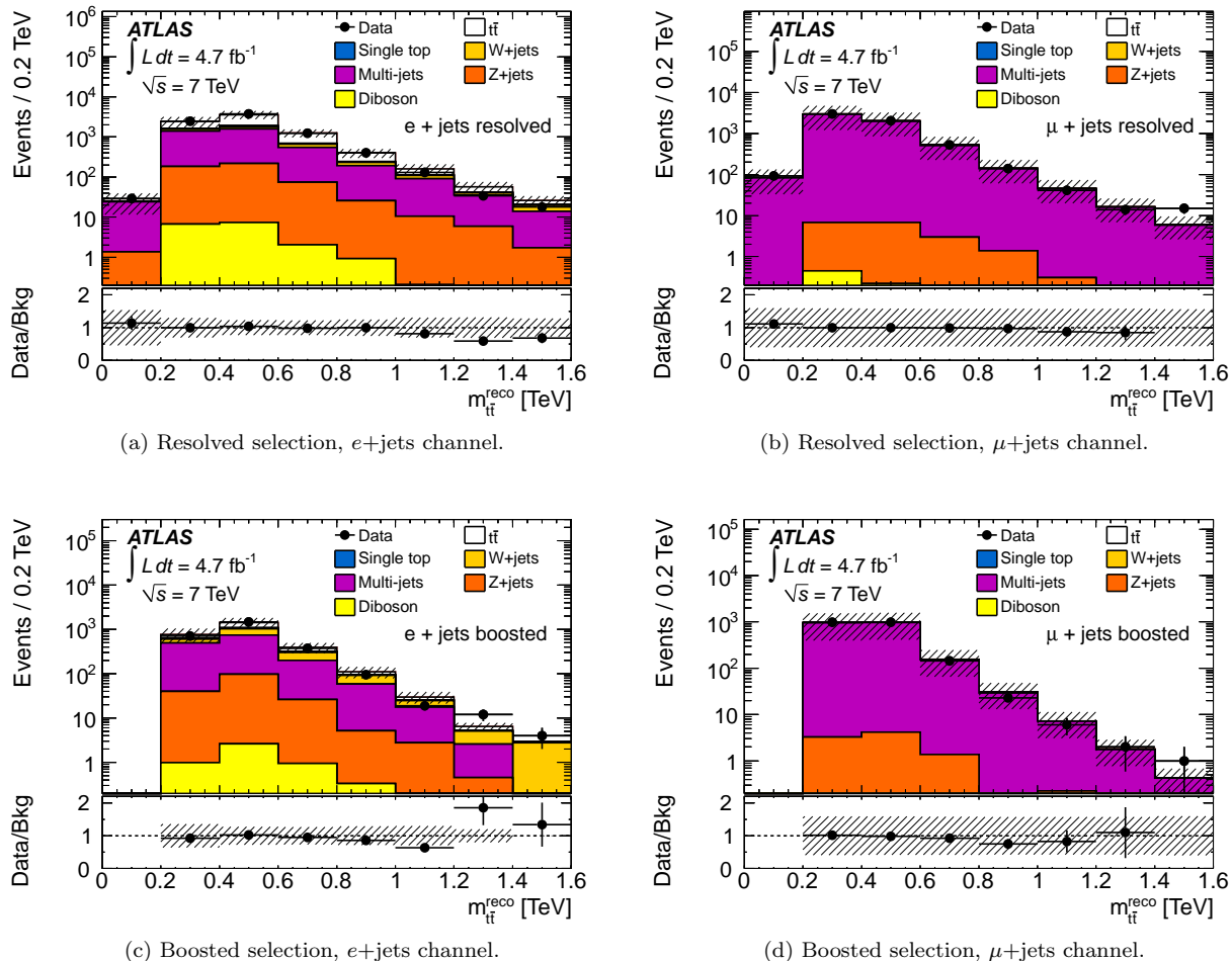
FIG. 3. The reconstructed t\bar{t} invariant mass, m_{t\bar{t}}^{\text{reco}} , in the multi-jet control regions for the resolved (a, b) and boosted (c, d) selections. The 60% uncertainty on the multi-jet contribution is indicated as the shaded area. The multi-jet fraction is significantly larger for the \mu + \text{jets} channel than for the e + \text{jets} channel because of the impact parameter requirement on the muons, which suppresses prompt muons.
