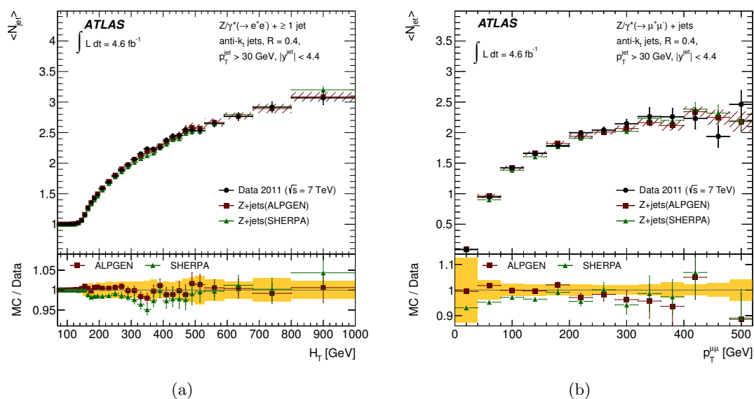
Figure 16. (a) Average number of jets, \langle N_{\text{jet}} \rangle , in Z (\rightarrow ee) + \text{jets} events as a function of the scalar p_T sum of the leptons and the jets, H_T , and (b) average number of jets in Z (\rightarrow \mu\mu) + \text{jets} events as a function of the transverse momentum of the Z boson candidate, p_T^{\text{ll}} , measured in data and predicted by the generators ALPGEN and SHERPA (see legend for details). The data points indicate the measured distribution after subtraction of electroweak and multi-jet background. The hatched band corresponds to the combined statistical and systematic uncertainty on the Z+jets prediction, modelled with ALPGEN. The error bars on each data point show the combined statistical and systematic uncertainty on the data. The bottom panel shows the MC/data ratio. The shaded band corresponds to the total systematic uncertainty and the error bars to the statistical uncertainty on the MC/data ratio.
