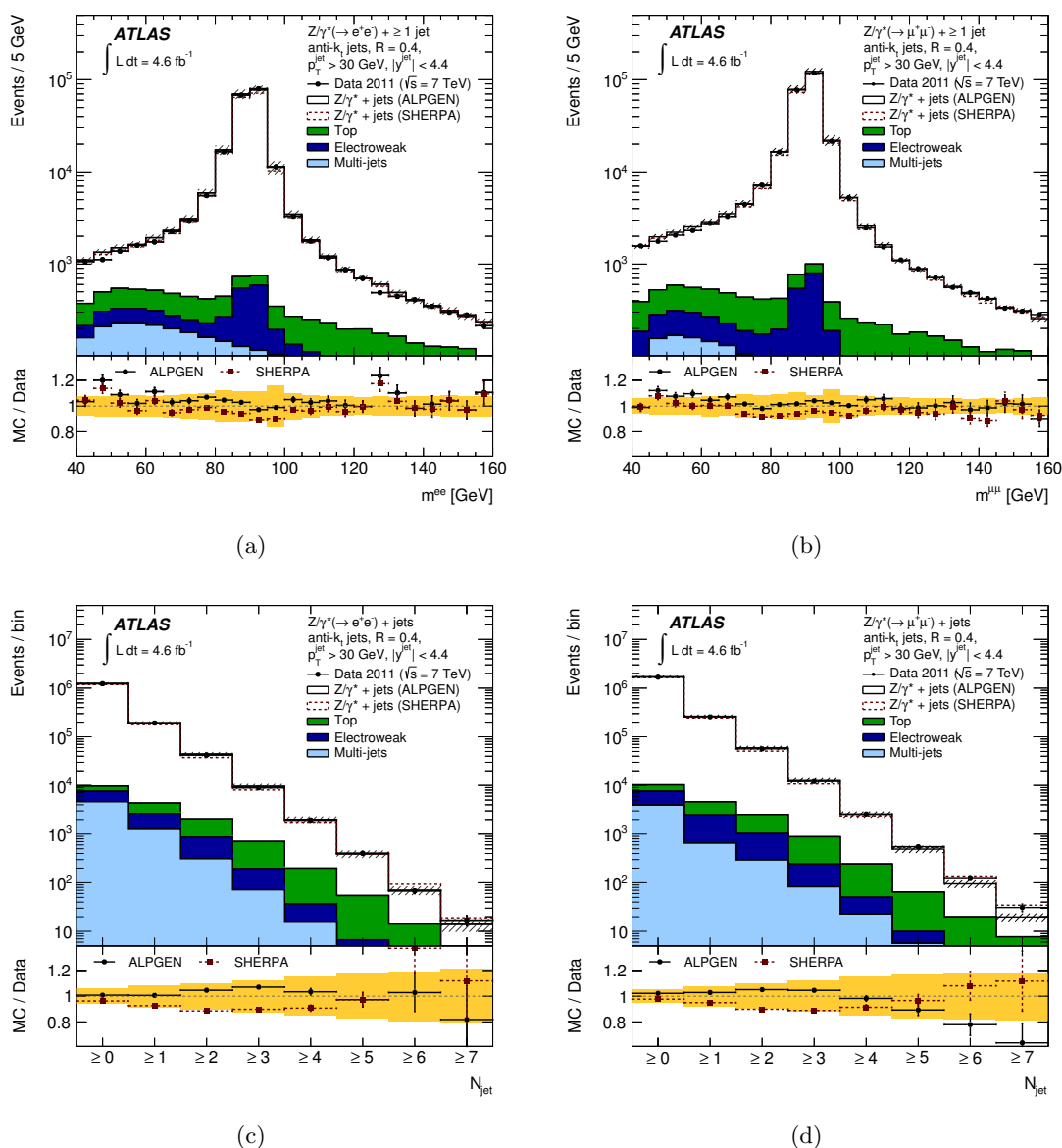
Figure 1. Numbers of events observed in data and predicted in simulation that pass the Z(\rightarrow ee) +jets and Z(\rightarrow \mu\mu) +jets selection as a function of the invariant mass of the Z candidate, (a) m^{ee} and (b) m^{\mu\mu} , for events with at least one jet with p_T^{\text{jet}} > 30 GeV and |y^{\text{jet}}| < 4.4 , and as a function of the inclusive jet multiplicity, N_{\text{jet}} , in (c) di-electron and (d) di-muon events. The individual contributions of the various backgrounds are also shown, as detailed in the legend. The hatched band corresponds to the combined statistical and systematic uncertainty on the prediction, obtained using ALPGEN to model the Z +jets process. The error bars on each data point show the statistical uncertainty. The bottom panel shows the corresponding MC/data ratio. The shaded band corresponds to the total systematic uncertainty and the error bars to the statistical uncertainty on the MC/data ratio.
