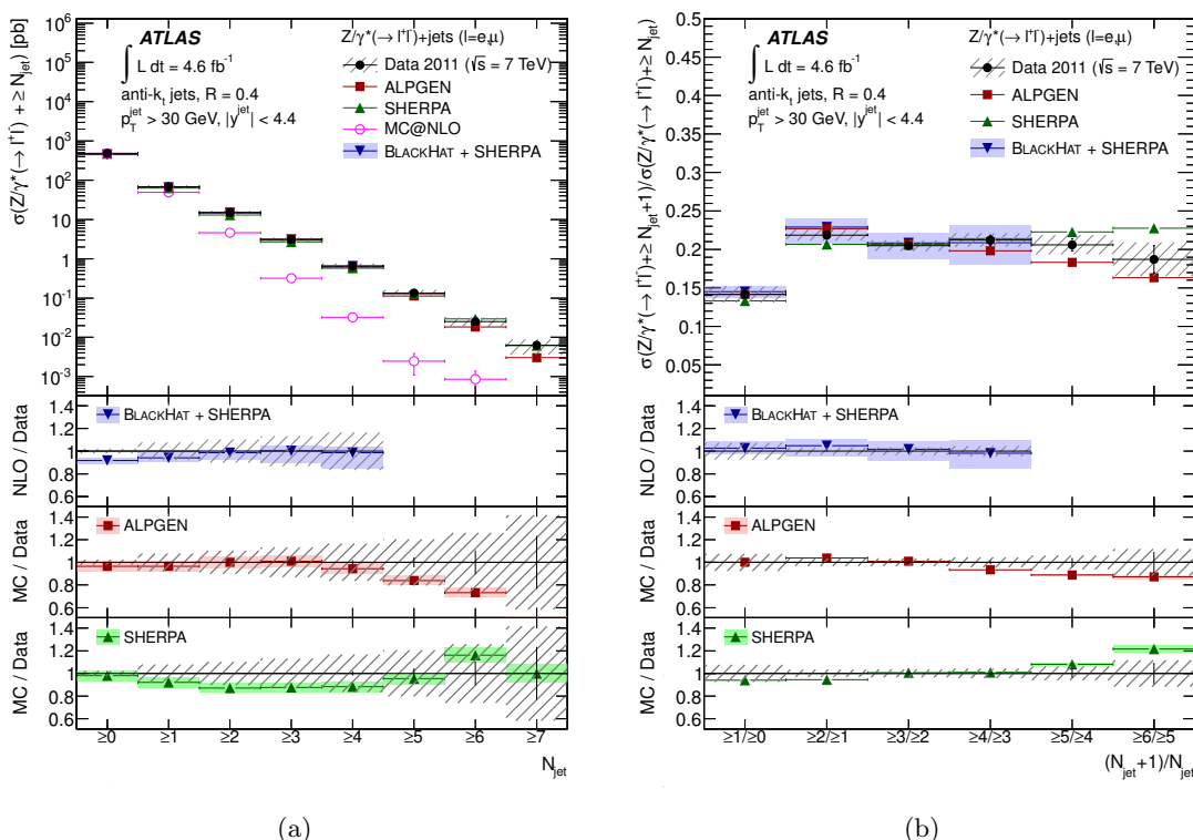
Figure 2. (a) Measured cross section for Z(\rightarrow\ell\ell)+\text{jets} as a function of the inclusive jet multiplicity, N_{\text{jet}} , and (b) ratio of cross sections for successive inclusive jet multiplicities. The data are compared to NLO pQCD predictions from BLACKHAT+SHERPA corrected to the particle level, and the ALPGEN, SHERPA and MC@NLO event generators (see legend for details). The error bars indicate the statistical uncertainty on the data, and the hatched (shaded) bands the statistical and systematic uncertainties on data (prediction) added in quadrature.
