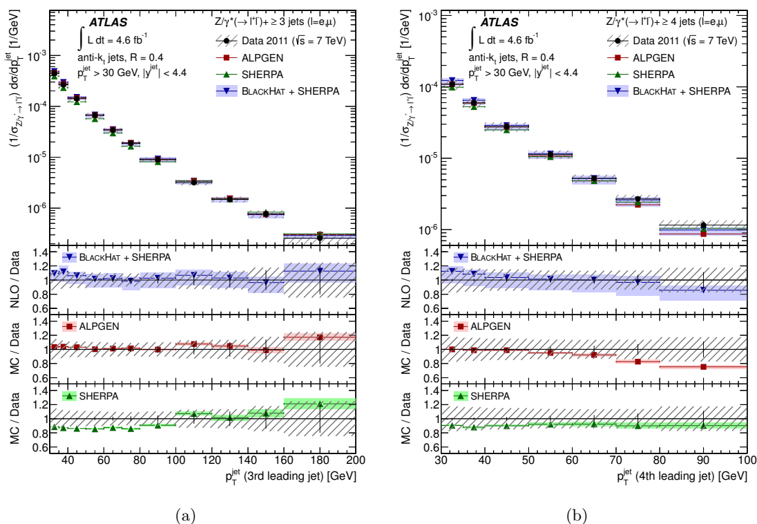
Figure 6. (a) Measured cross section for Z(\rightarrow \ell\ell) + \text{jets} as a function of the transverse momentum, p_T^{\text{jet}} , of the third leading jet for events with at least three jets with p_T^{\text{jet}} > 30 GeV and |y^{\text{jet}}| < 4.4 in the final state and (b) as a function of p_T^{\text{jet}} of the fourth leading jet for events with at least four jets. The cross sections are normalized to the inclusive Z(\rightarrow \ell\ell) cross section. The other details are as in figure 2.
