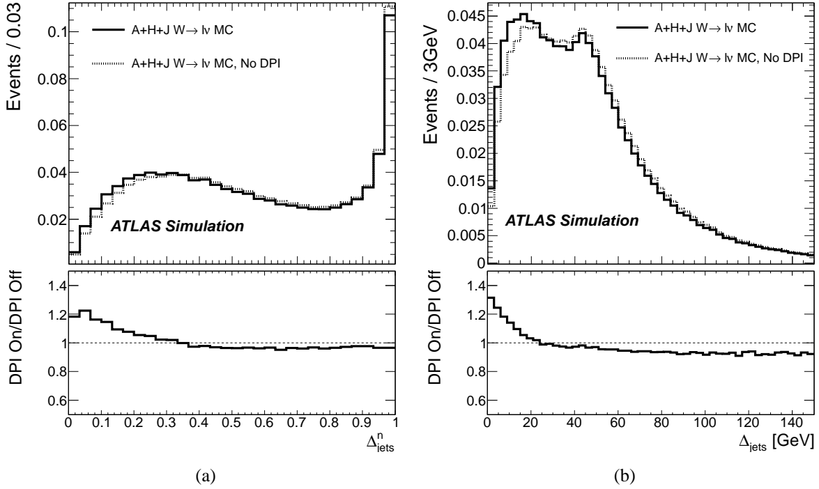
Figure 3. Comparison of the shapes of (a) \Delta_{jets}^n and (b) \Delta_{jets} distributions, at detector level, for selected W \rightarrow \ell\nu + 2\text{-jet} events as expected in A+H+J, with DPI on and off (Template A). The lower panels show the respective ratios of the DPI-on and DPI-off expectations.
