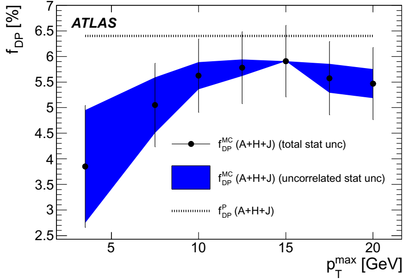
Figure 5. Variation of the extracted fraction of double-parton scattering from the \Delta_{\text{jets}}^n distribution in the A + H + J MC simulation, f_{DP}^{(MC)} (black points), as a function of the transverse momentum cut imposed on the scattered partons, p_T^{\max} . The band illustrates the statistical component of the uncertainty of f_{DP}^{(MC)} , relative to the reference sample with p_T^{\max} = 15 GeV, estimated by subtracting the statistical uncertainty of the reference sample in quadrature. The value, f_{DP}^{(P)} , of the fraction of double-parton scattering obtained directly at the parton level (see equation (16)) is also shown as a dashed line.
