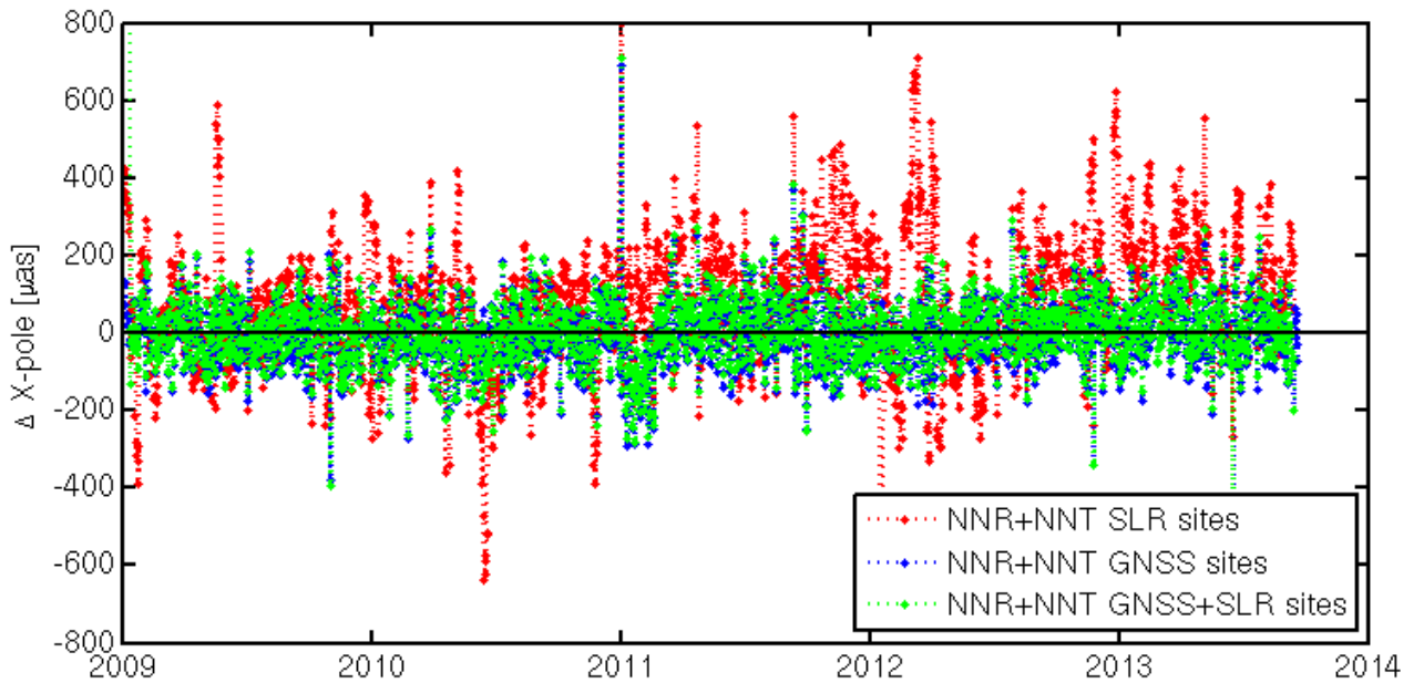
Figure 4. Estimated x-pole coordinates w.r.t. IERS-08-C04 using different sets of core sites for the datum definition (i.e., NNR and NTT conditions w.r.t. ITRF2008).
