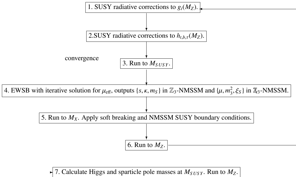
Figure 1: Iterative algorithm used to calculate the NMSSM spectrum. The initial step is the uppermost one. M_{SUSY} is the scale at which the EWSB conditions are imposed, as discussed in the text. M_X is the scale at which the high energy SUSY breaking boundary conditions are imposed. Although Higgs and sparticle masses are calculated at M_{SUSY} , the empirical values of electroweak boson and quark/lepton masses are imposed at M_Z . It is the SOFTSUSY convention to evolve \overline{DR} couplings to M_Z as the final step, although in the SLHA2 output [35], various couplings at M_{SUSY} are output.
