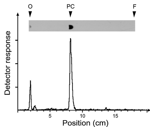
Fig. 1. Biosynthesis of [ 3 H]PC in T. brucei . Procyclic form trypanosomes (4 × 10 7 parasites) were incubated in the presence 1 μCi/ml [ 3 H]choline for 2 h in 5 ml culture medium. Phospholipids were extracted using organic solvents and separated by TLC. [ 3 H]-labeled lipids were analyzed by radioisotope scanning, and fluorography (inset). The arrows refer to the migration of a phosphatidylcholine (PC) standard run on the same TLC plate. The site of sample application (O) and the migration distance of the solvent front (F) are indicated.
