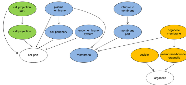
Figure 5 Cellular component analysis of potential pathogenicity factors from N. fowleri . Gene Ontology (GO) graph generated from the cellular component ontology of the proteins, which were up-regulated in highly pathogenic trophozoites compared to weakly pathogenic trophozoites. The specificity of the GO terms increases from the bottom to the top of the graph with arrows indicating "being part of". The majority of the potential pathogenicity factors localize to the membrane of the cell (blue marked circles), whereas another group of proteins localized to either cell projections (green marked circles) or vesicles (orange marked circles).
