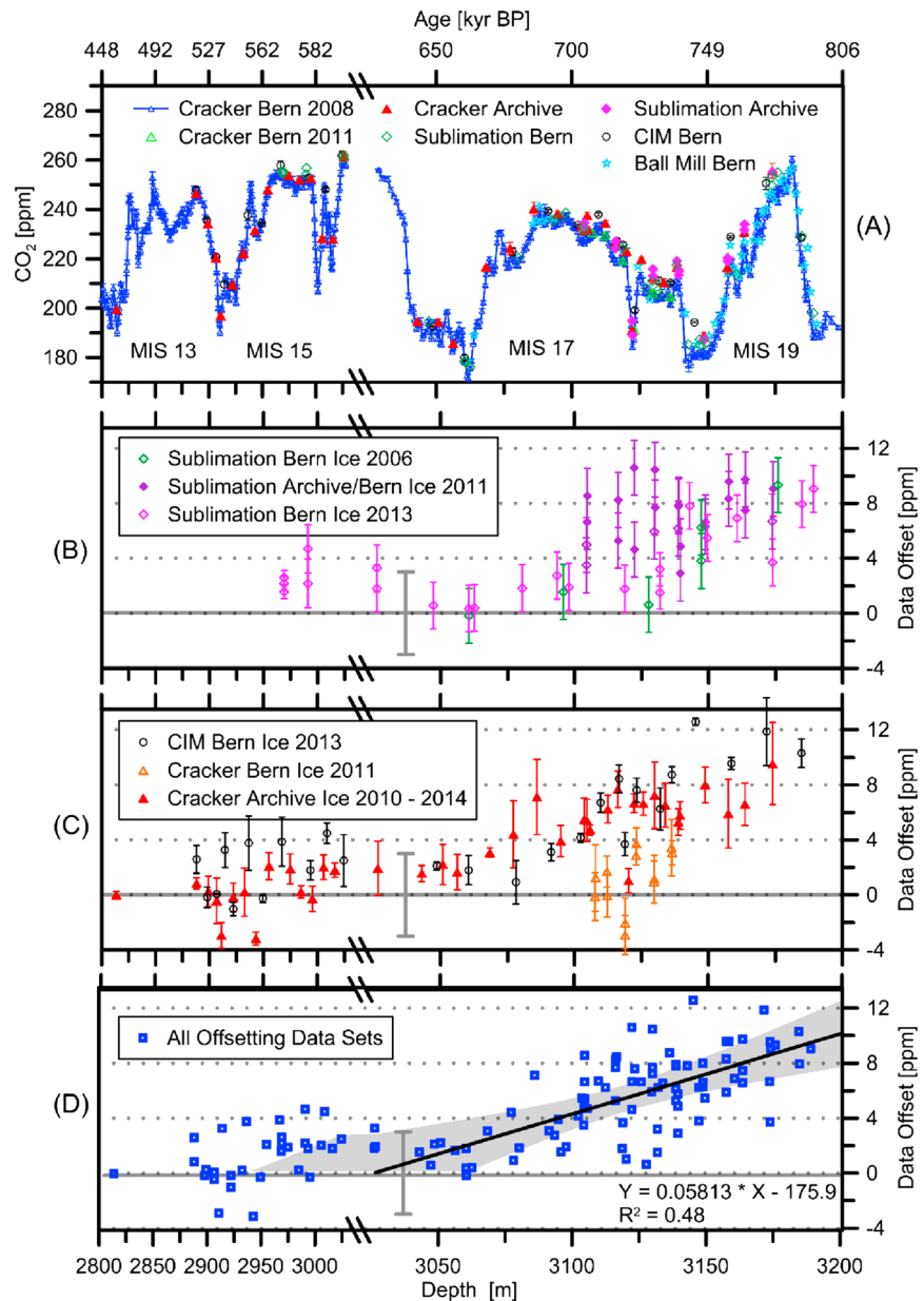
Figure 1. (a) Compilation of EDC CO 2 data between 2800 m and 3200 m depth (442–816 kyr B.P. based on AICC2012 [Bazin et al., 2013]). The original data published by Siegenthaler et al. [2005] and Lüthi et al. [2008] using the cracker (dark blue triangles), or the ball mill (light blue stars) system, and Bern ice are shown. The cracker data were found to be slightly lower than the ball mill data, which is likely an artifact of the extraction bias shown here (see supporting information). The other data are remeasurements of this study and Schneider [2011] (Sublimation 2011) using different types of ice and analytical systems according to the following codes: closed symbols: archive ice stored at Dome C at -53.5 \pm 10^\circ\text{C} , open symbols: ice stored in Bern/Grenoble (Bern ice) at laboratory freezer temperatures ( -22.5 \pm 2.5^\circ\text{C} ), triangles: data obtained with the cracker, diamonds: data obtained with the sublimation, and bullets: data obtained with the CIM. Marine oxygen isotope stages (MIS) 13–19 are marked for reference. (b–d) Offsets between original EDC cracker CO 2 records [Siegenthaler et al., 2005; Lüthi et al., 2008] and remeasurements, expressed as current measurements minus previously published cracker values. Depending on the depth of the remeasurement relative to the cracker data, either the nearest or the average of the two neighboring cracker data points is used as reference. The error bar at 3030 m depth represents the estimated range within which a single remeasurement cannot be attributed as being significantly different from the zero line ( \pm 3 ppm), since ice samples could not be taken from exactly the same depth. Note that this error does not account for possible systematic uncertainties in the range of \pm 2 ppm between the different analytical systems. In Figures 1b and 1c, the same symbol coding is used as in Figure 1a with the addition in the legend of the years at which the corresponding data set was obtained. In Figure 1d, the compilation of all remeasurements that indicate an offset (all data from Figures 1b and 1c with the exception of Cracker Bern 2011) is shown, including the best estimate correction curve (black line and linear equation) and its 95% uncertainty range (gray area) (see text for more details). Note the break in the horizontal axes.
