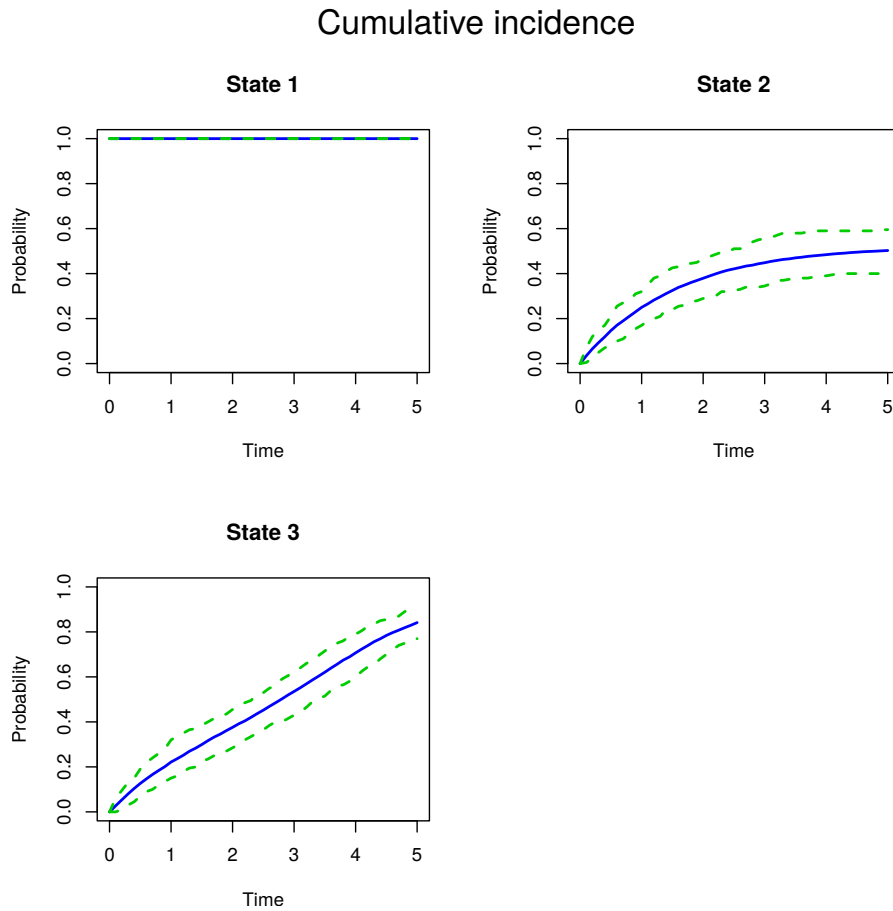
Figure 5: Cumulative incidence.
