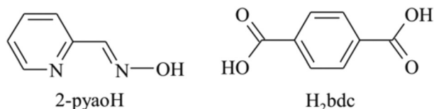
Scheme 2 Schematic illustration of the ligands with acronyms used in this study.
