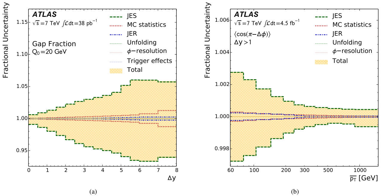
Fig. 2: Summary of systematic uncertainties on (a) the gap fraction as a function of \Delta y and (b) the \langle \cos(\pi - \Delta\phi) \rangle distribution as a function of \overline{p_T} . Here the systematic uncertainties from the jet energy scale (dark dashes), Monte Carlo statistical precision (dark dots), jet energy resolution as (dark dashed-dots), unfolding (light dashes), jet \phi resolution (light dots) and from residual trigger inefficiencies (light dashed-dots) are shown. The total systematic uncertainty (light cross-hatched area) is also shown.
