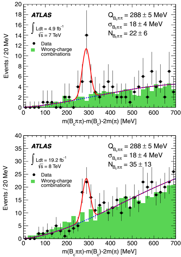
FIG. 2 (color online). The Q = m(B_c^\pm \pi\pi) - m(B_c^\pm) - 2m(\pi^\pm) distribution for the right-charge combinations (points with error bars) and for the same (wrong) pion charge combinations (shaded histogram) in 7 TeV data (top) and in 8 TeV data (bottom). The wrong-charge combinations are normalized to the same yield as the right-charge background. The solid line is the projection of the results of the unbinned maximum likelihood fit to all candidates in the range 0–700 MeV. The dashed line is the projection of the background component of the same fit.
