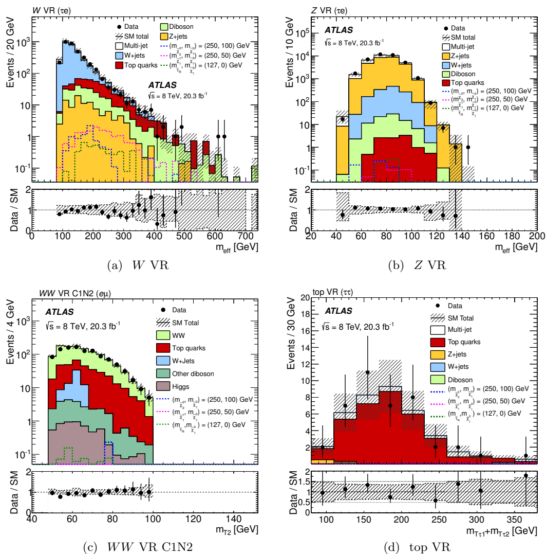
Figure 5. Distributions of relevant kinematic variables in the validation regions: m_{\text{eff}} in the (a) W and (b) Z VRs, (c) m_{T2} in the WW VR C1N2, and (d) m_{T\tau1} + m_{T\tau2} in the top VR. In the Z VR, events containing one electron and one tau are shown. The SM backgrounds other than multi-jet production are estimated from MC simulation and normalised to 20.3 \text{ fb}^{-1} . The hatched bands represent the combined statistical and systematic uncertainties on the total SM background. For illustration, the distributions of the SUSY reference points are also shown as dashed lines. The lower panels show the ratio of data to the SM background estimate.
