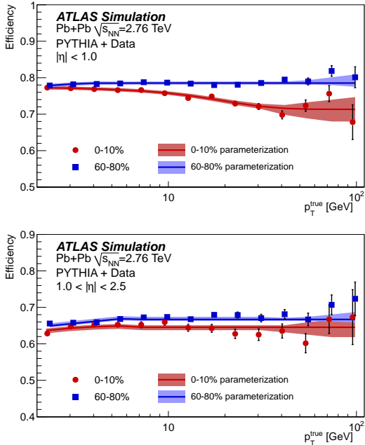
Figure 2: Charged-particle reconstruction efficiency as a function of truth p_T , for 0–10% (red) and 60–80% (blue) centrality bins in the region |\eta| < 1 (top) and 1 < |\eta| < 2.5 (bottom). The p_T values for the 0–10% points are shifted for clarity. The solid curves show parameterizations of efficiencies. The shaded bands show the systematic uncertainty in the parameterized efficiencies (see text).
