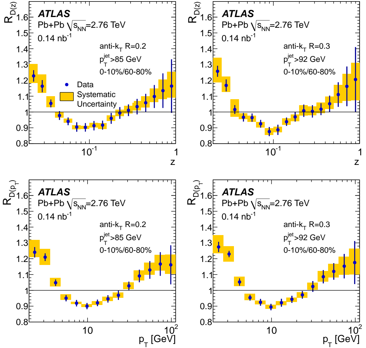
Figure 8: Ratios of unfolded fragmentation functions, D(z) (top) and D(p_T) (bottom), for central (0–10%) collisions to those in peripheral (60–80%) collisions for R = 0.2 (left) and R = 0.3 (right) jets. The fragmentation functions were evaluated using charged hadrons within \Delta R = 0.4 of the jet axis. The error bars on the data points indicate statistical uncertainties while the yellow shaded bands indicate systematic uncertainties.
