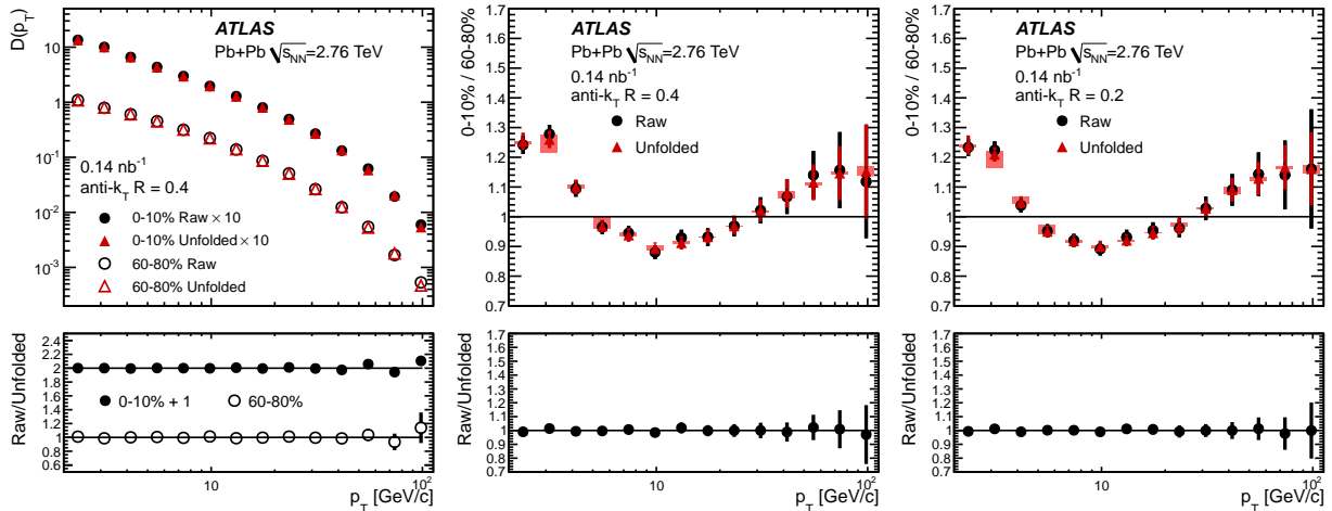
Figure 4: Measured and unfolded D(p_T) distributions for R = 0.4 and R = 0.2 jets in central (0–10%) and peripheral (60–80%) collisions. Top left: R = 0.4 D^{\text{meas}}(p_T) and D(p_T) distributions, bottom left: ratios of measured to unfolded R = 0.4 D(p_T) distributions with the 0–10% shifted by +1 for clarity. Top middle and right: central-to-peripheral ratios of measured ( R_{D(p_T)}^{\text{meas}} ) and unfolded ( R_{D(p_T)} ) distributions for R = 0.4 and R = 0.2 , respectively. Bottom middle and right: ratio of R_{D(p_T)}^{\text{meas}} to R_{D(p_T)} for R = 0.4 and R = 0.2 , respectively.
