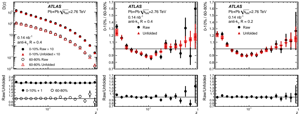
Figure 3: Measured and unfolded D(z) distributions for R = 0.4 and R = 0.2 jets in central (0–10%) and peripheral (60–80%) collisions. Top left: R = 0.4 D^{\text{meas}}(z) and D(z) distributions, bottom left: ratios of measured to unfolded R = 0.4 D(z) distributions with the 0–10% shifted by +1 for clarity. Top middle and right: central-to-peripheral ratios of measured ( R_{D(z)}^{\text{meas}} ) and unfolded ( R_{D(z)} ) distributions for R = 0.4 and R = 0.2 , respectively. Bottom middle and right: ratio of R_{D(z)}^{\text{meas}} to R_{D(z)} for R = 0.4 and R = 0.2 , respectively.
