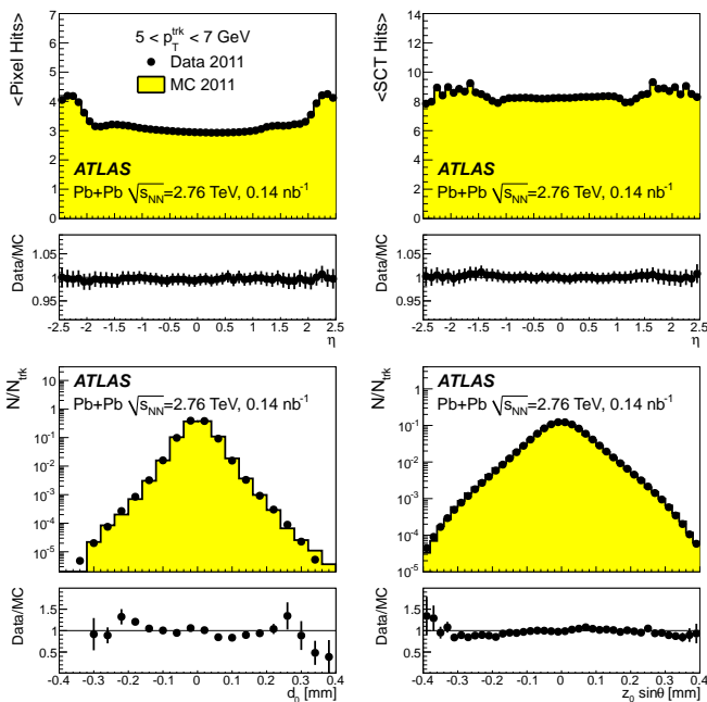
Figure 1: Comparison between data and MC distributions for four different charged-particle reconstruction selection parameters. The distributions are shown for the 0–10% centrality bin and for charged-particle transverse momenta in the range 5 < p_T^{\text{ch}} < 7 GeV. Top: average number of pixel (left) and SCT (right) hits per track. Bottom: distribution of track impact parameters with respect to the reconstructed primary vertex; both transverse, d_0 (left), and longitudinal, z_0 \sin \theta (right), impact parameters are shown. Ratios of distributions in data to those in MC simulation are shown for each quantity.
