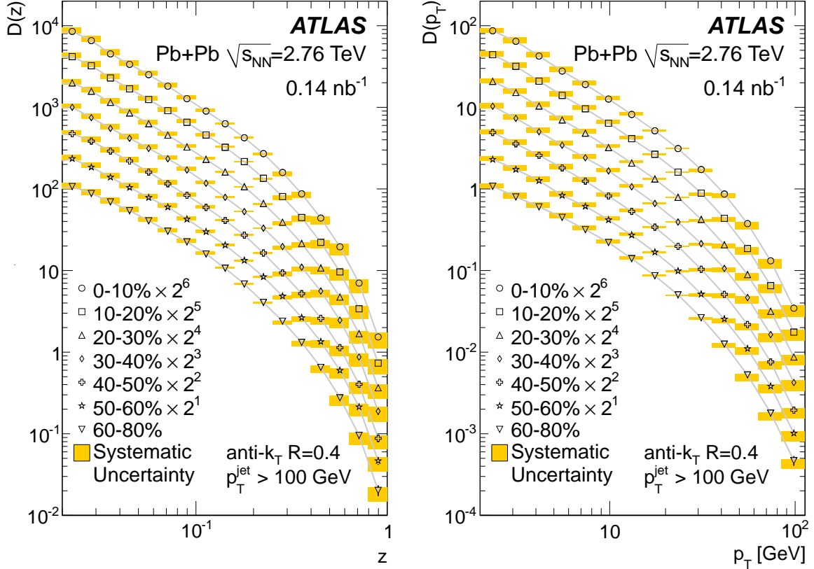
Figure 5: Unfolded R = 0.4 longitudinal charged particle fragmentation function, D(z) and the charged particle transverse momentum distribution, D(p_T) , for the seven centrality bins included in this analysis. The statistical uncertainties are everywhere smaller than the points. The yellow shaded error bars indicate systematic uncertainties. Grey lines connecting the central values of distributions are to guide the eye.
