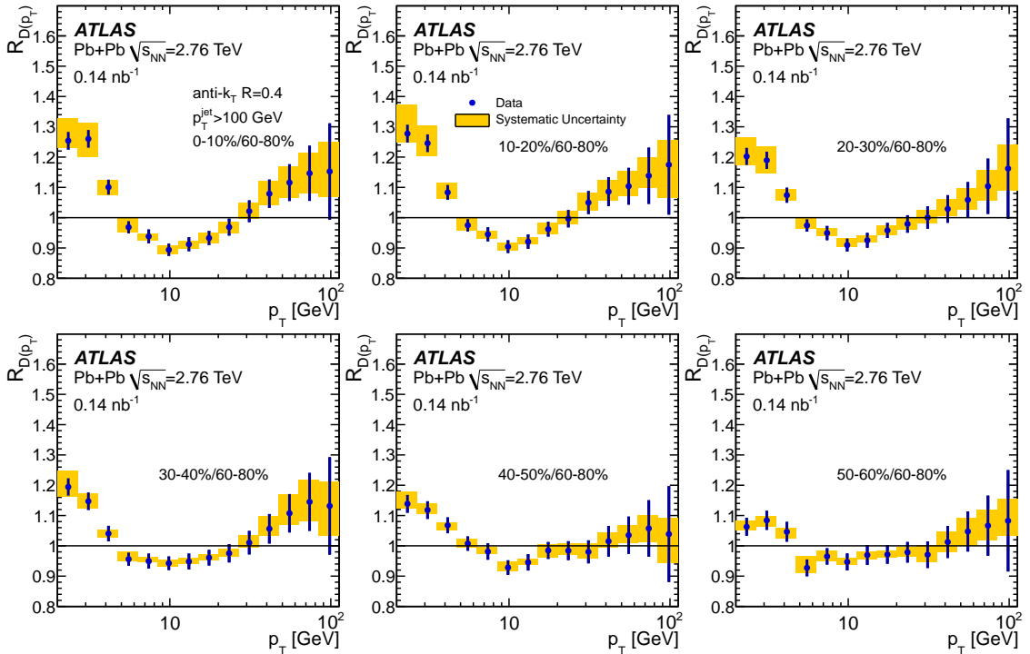
Figure 7: Ratios of unfolded D(p_T) distributions for six bins in collision centrality to those in peripheral (60–80%) collisions, D(p_T)|_{\text{cent}}/D(p_T)|_{60-80} , for R = 0.4 jets. The error bars on the data points indicate statistical uncertainties while the yellow shaded bands indicate systematic uncertainties.
