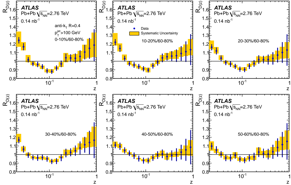
Figure 6: Ratios of D(z) for six bins in collision centrality to those in peripheral (60–80%) collisions, D(z)|_{\text{cent}}/D(z)|_{60-80} , for R = 0.4 jets. The error bars on the data points indicate statistical uncertainties while the yellow shaded bands indicate systematic uncertainties.
