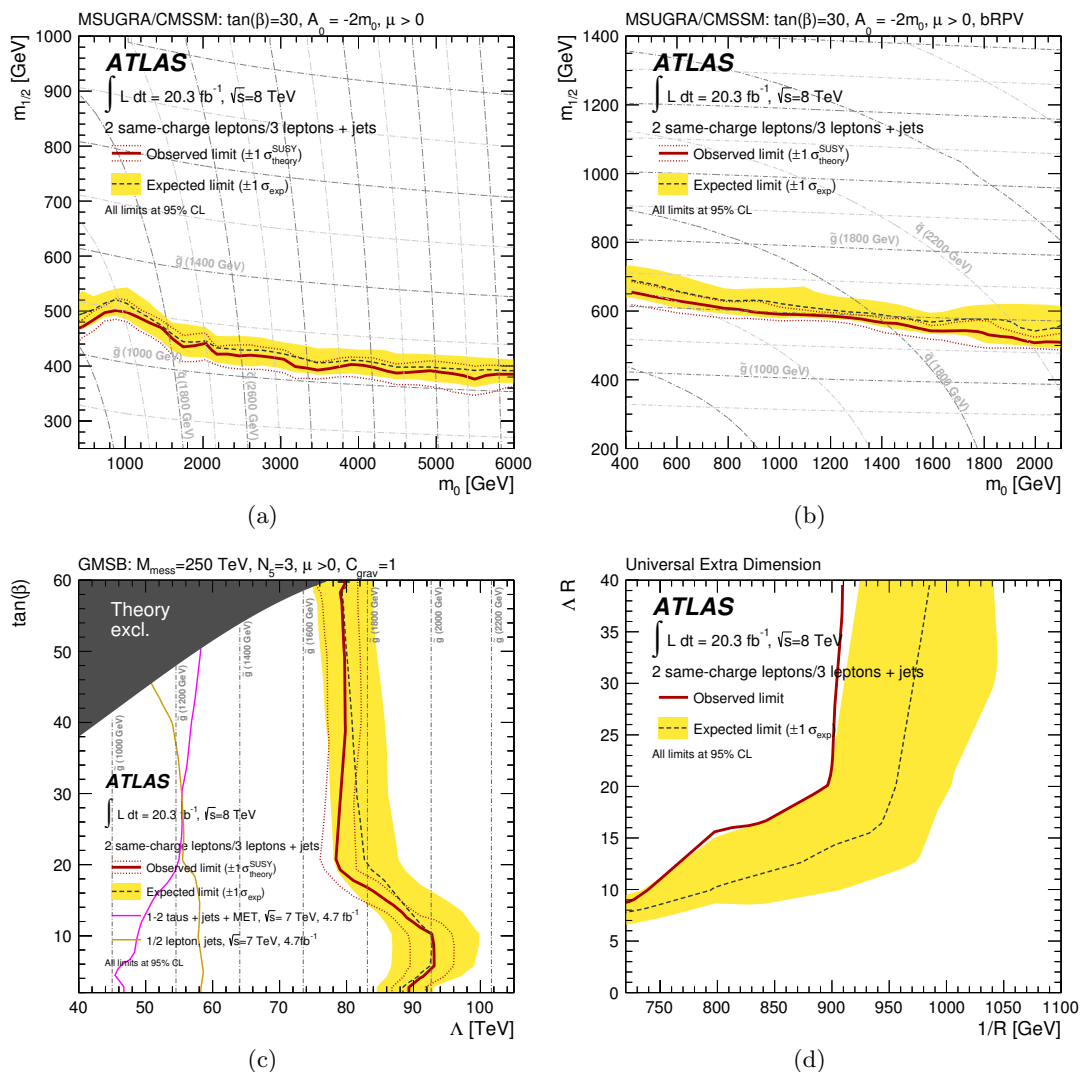
Figure 8. Observed and expected exclusion limits for the MSUGRA/CMSSM, bRPV, GMSB and mUED models, obtained with 20.3 \text{ fb}^{-1} of pp collisions at \sqrt{s}=8 TeV. When available, results are compared with the limits obtained by previous ATLAS searches [75, 77, 79].
