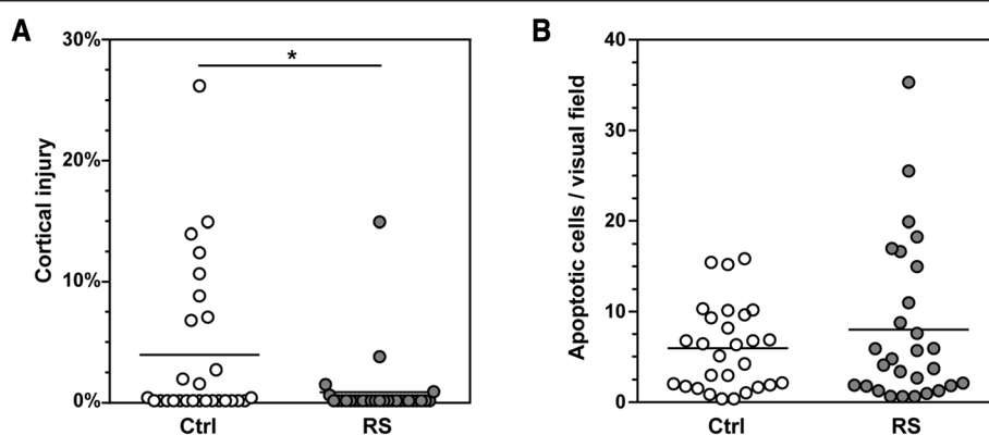
Figure 3 Brain injury 42 h after infection. (A) Statistically significant attenuation of cortical necrosis was seen in animals treated with the MMP inhibitor (RS) compared to littermates receiving the vehicle (Ctrl), while no effect was observed on hippocampal apoptosis (B) . * P < 0.05 (Mann-Whitney test).
