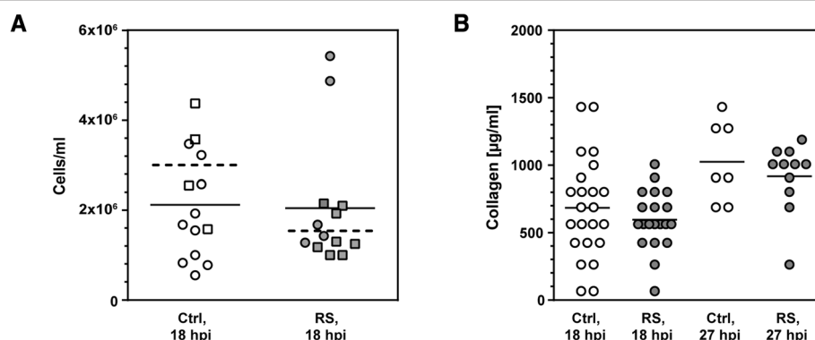
Figure 2 Measurements in samples of cerebrospinal fluid. (A) White blood cell count in cerebrospinal fluid samples obtained 18 h after infection (hours post infection (hpi)). No effect after pre-treatment with the MMP inhibitor (RS) was observed when compared to vehicle treated littermates (control (Ctrl)). Leukocyte counts were reduced after treatment with RS in the survivors of the disease ( P < 0.05 , Mann-Whitney test; squares). (B) Total collagen content was quantified at 18 and 27 hpi (optical density at 550 nm [OD 550 ] was used as arbitrary unit). Concentrations were lower in animals treated with RS compared to control littermates, although this effect did not reach statistical significance ( P = ns ).
